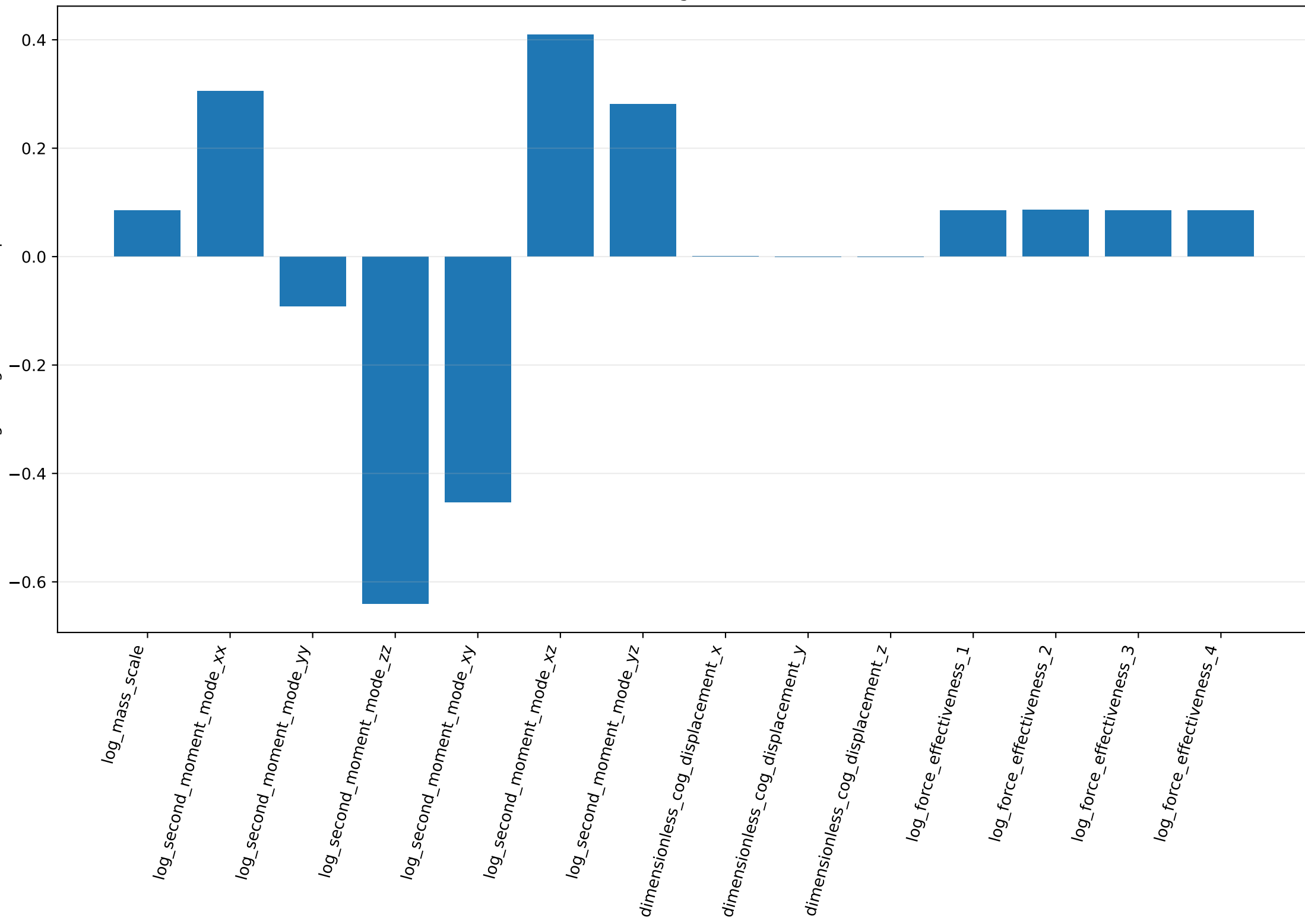
weak mode 12 / sigma=0.000574068
