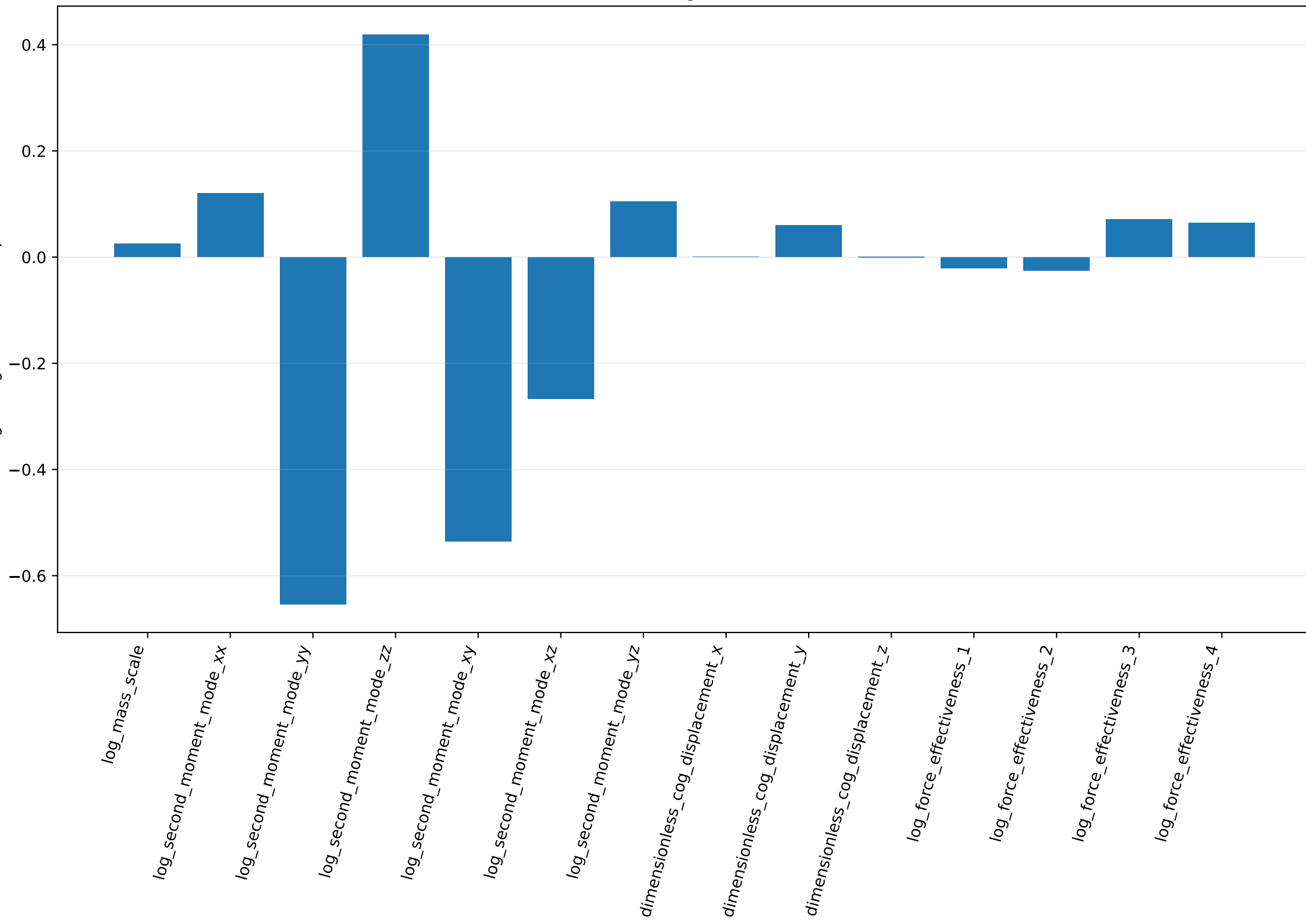
weak mode 11 / sigma=0.00393988
