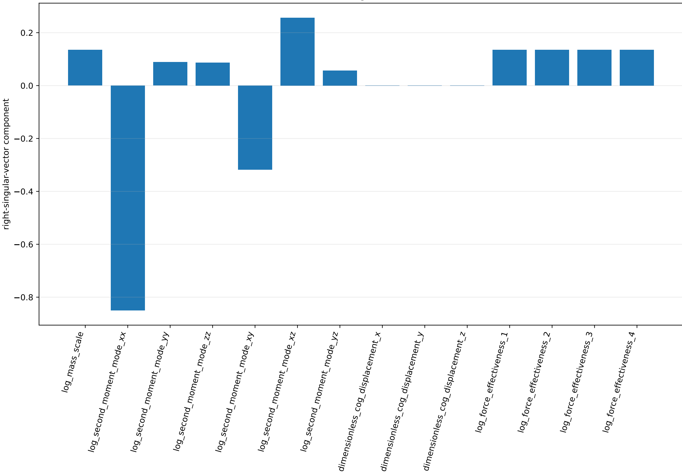
weak mode 13 / sigma=3.87005e-05
