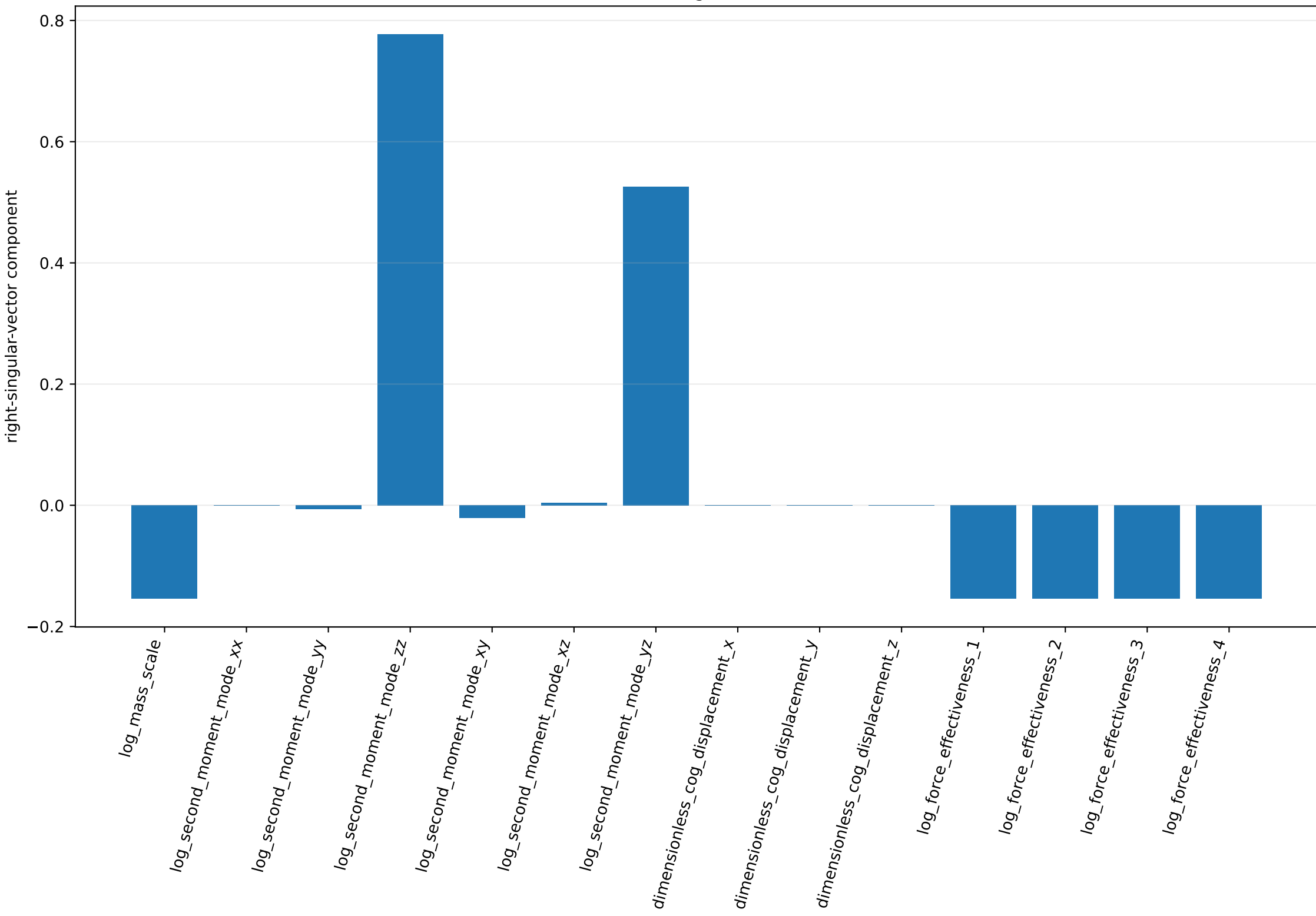
weak mode 12 / sigma=2.52245e-05
