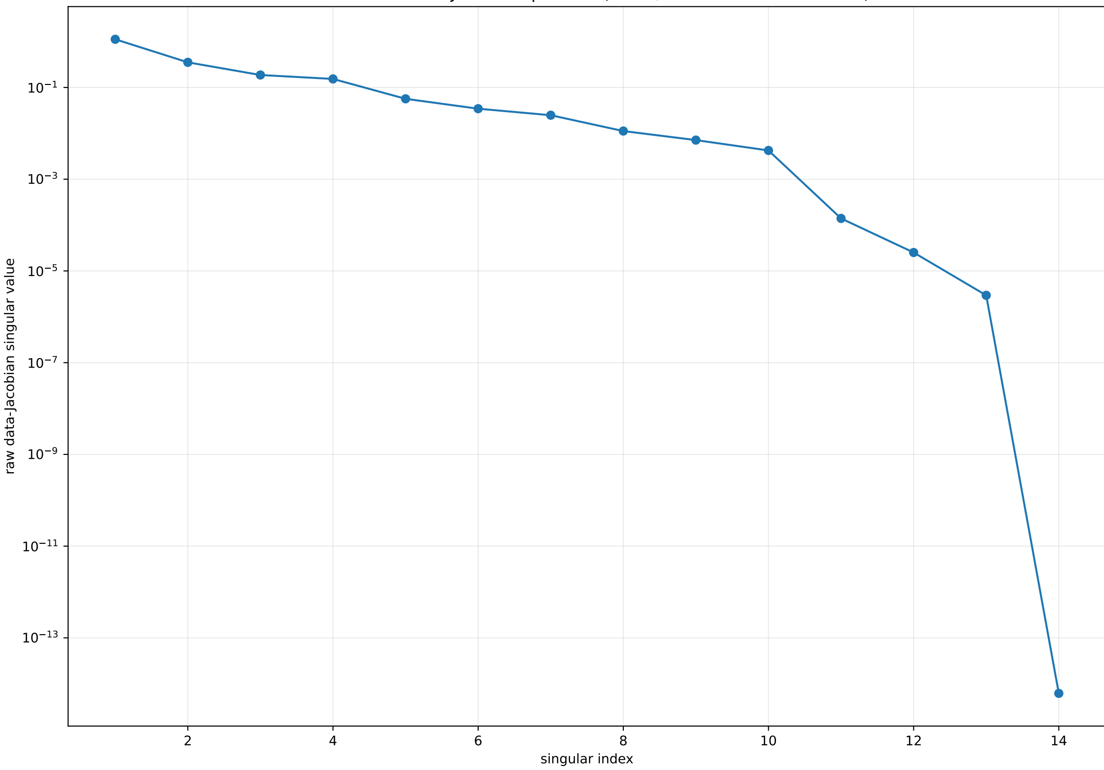
Raw deterministic Jacobian spectrum (no LM/KKT stabilization included)
