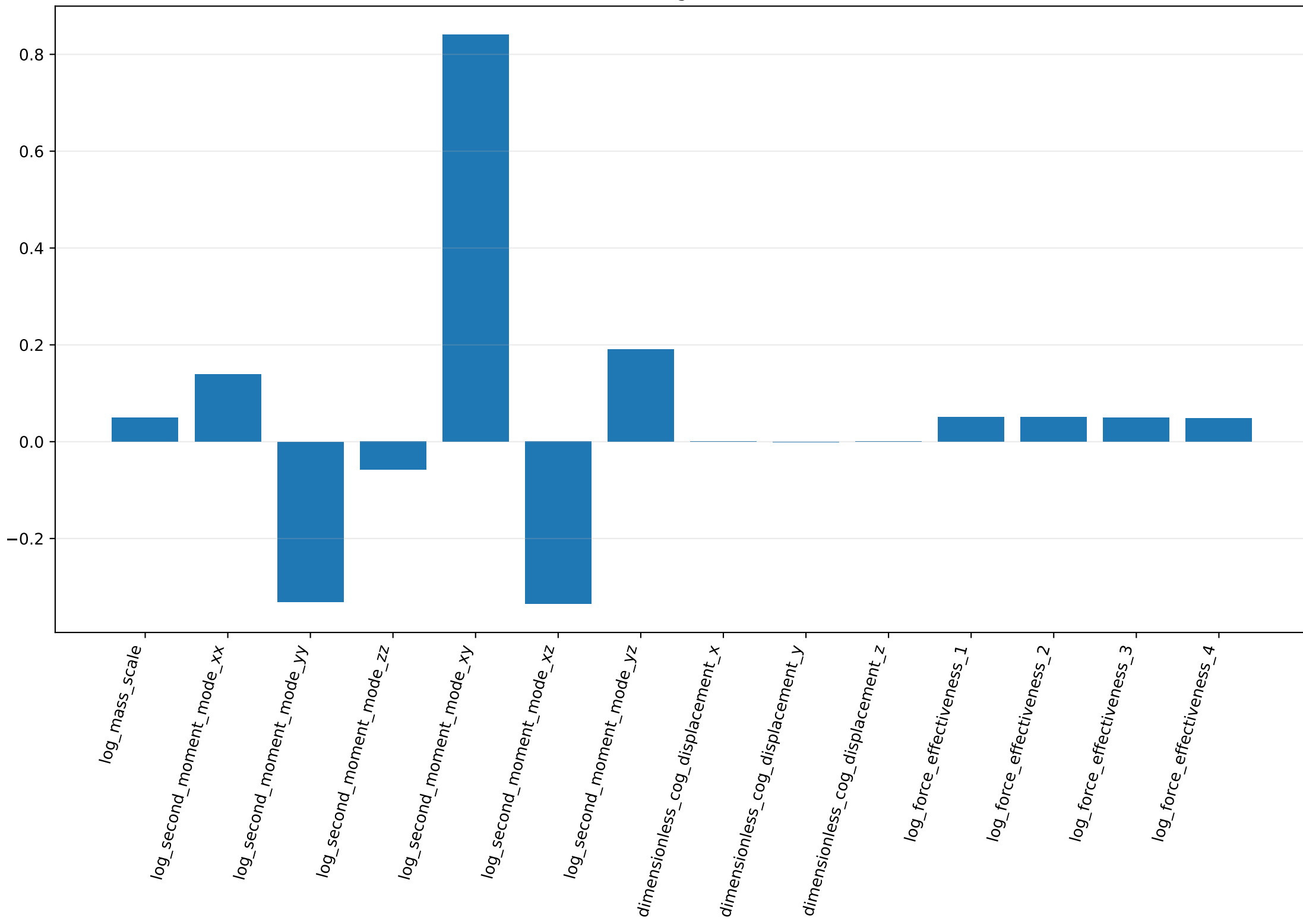
weak mode 11 / sigma=0.000139597
