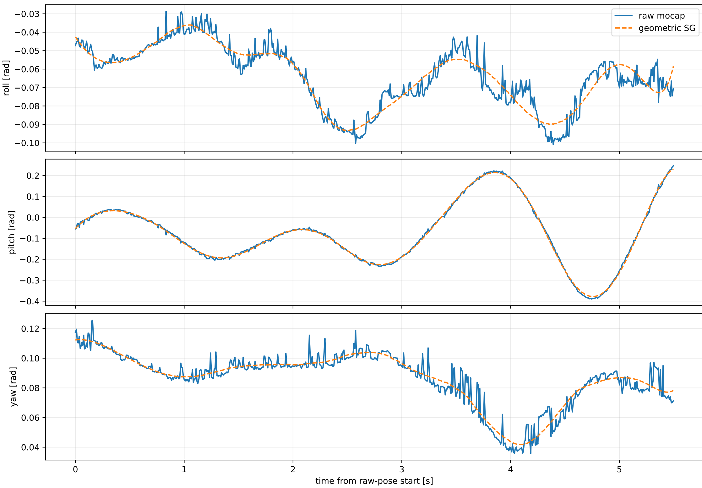
Raw mocap and geometric-SG orientation
