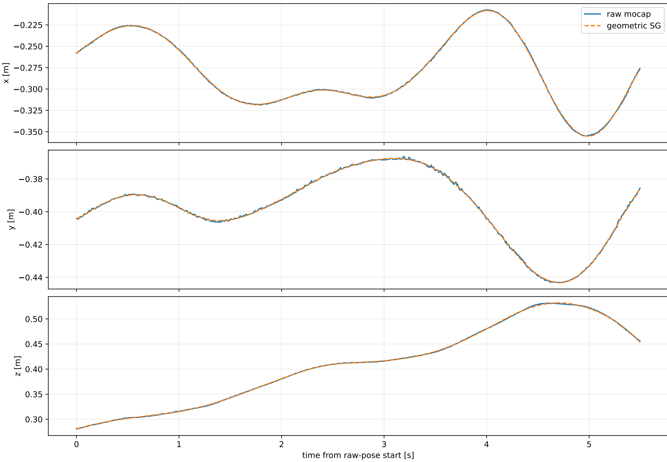
Raw mocap and geometric-SG position
