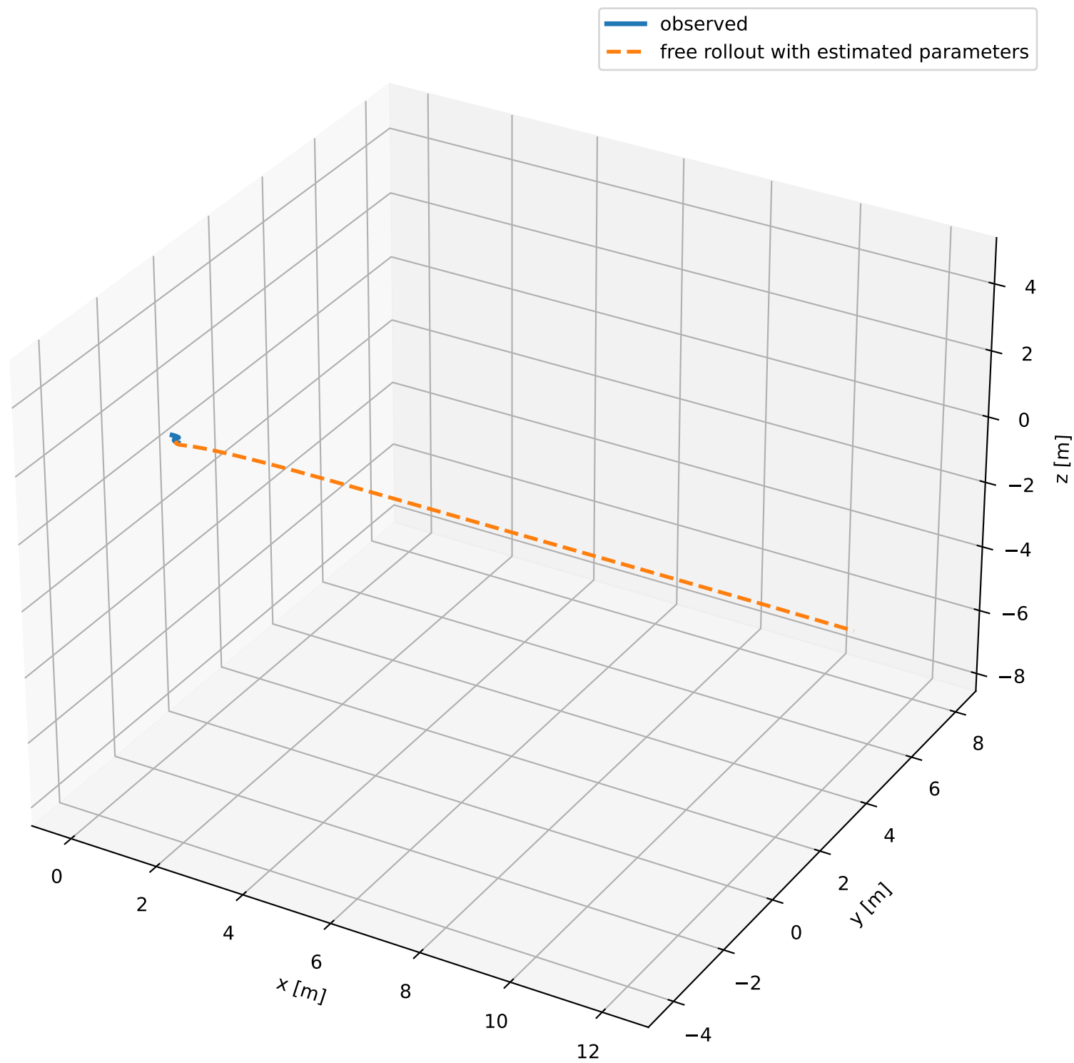
Observed and free-rollout 3D trajectory
