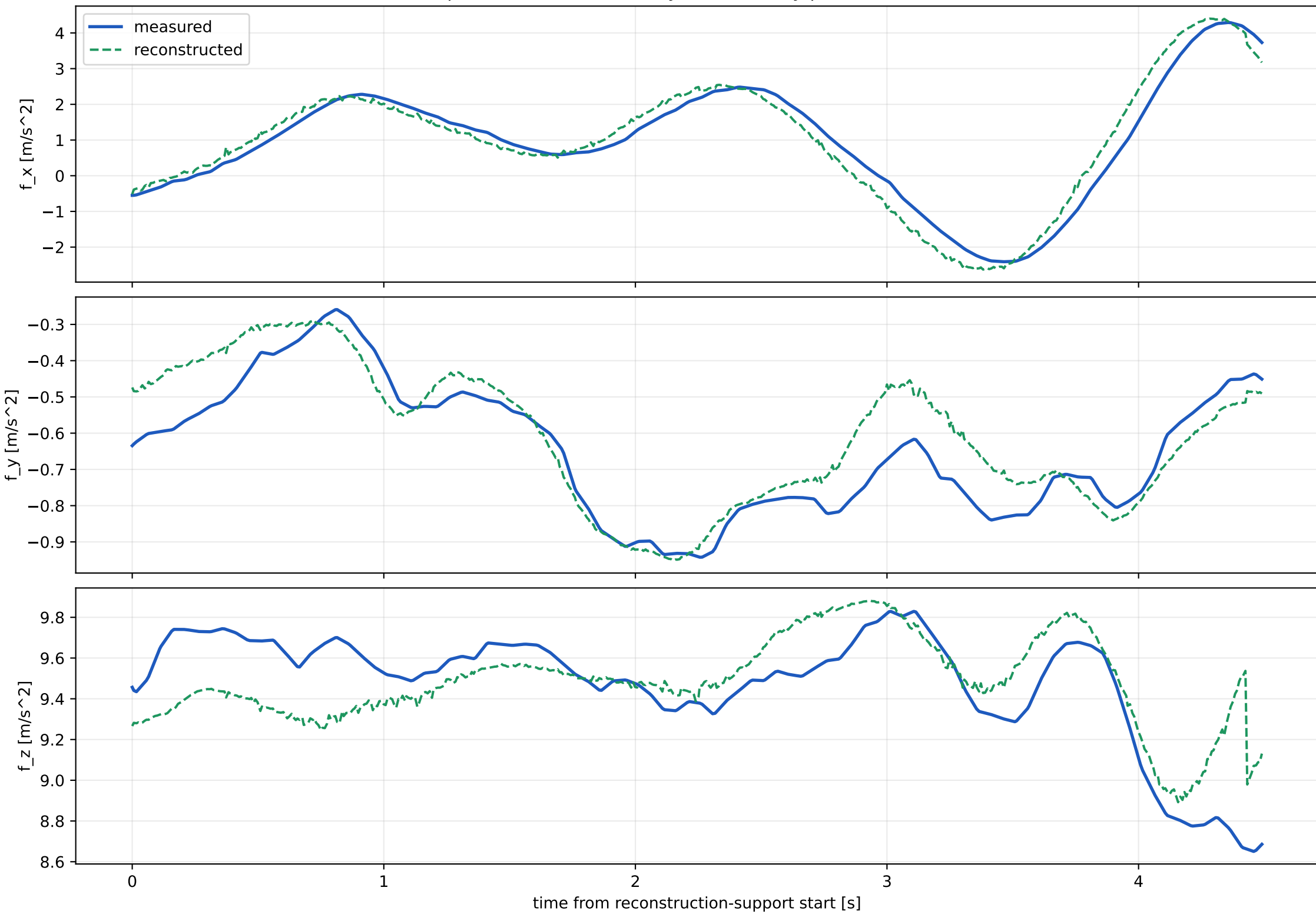
Specific force consistency (not used by parameter loss)
