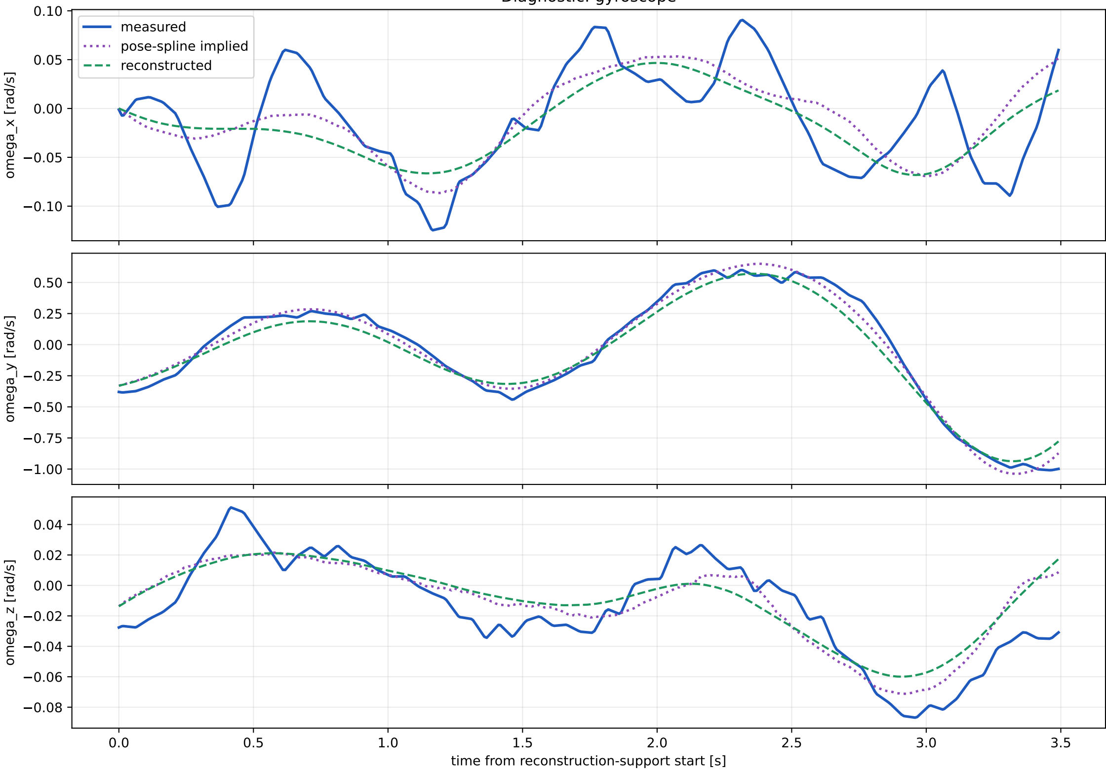
Diagnostic: gyroscope
