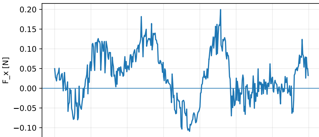
External-wrench diagnostic: raw inverse-dynamics residual (no external-wrench minimization)
