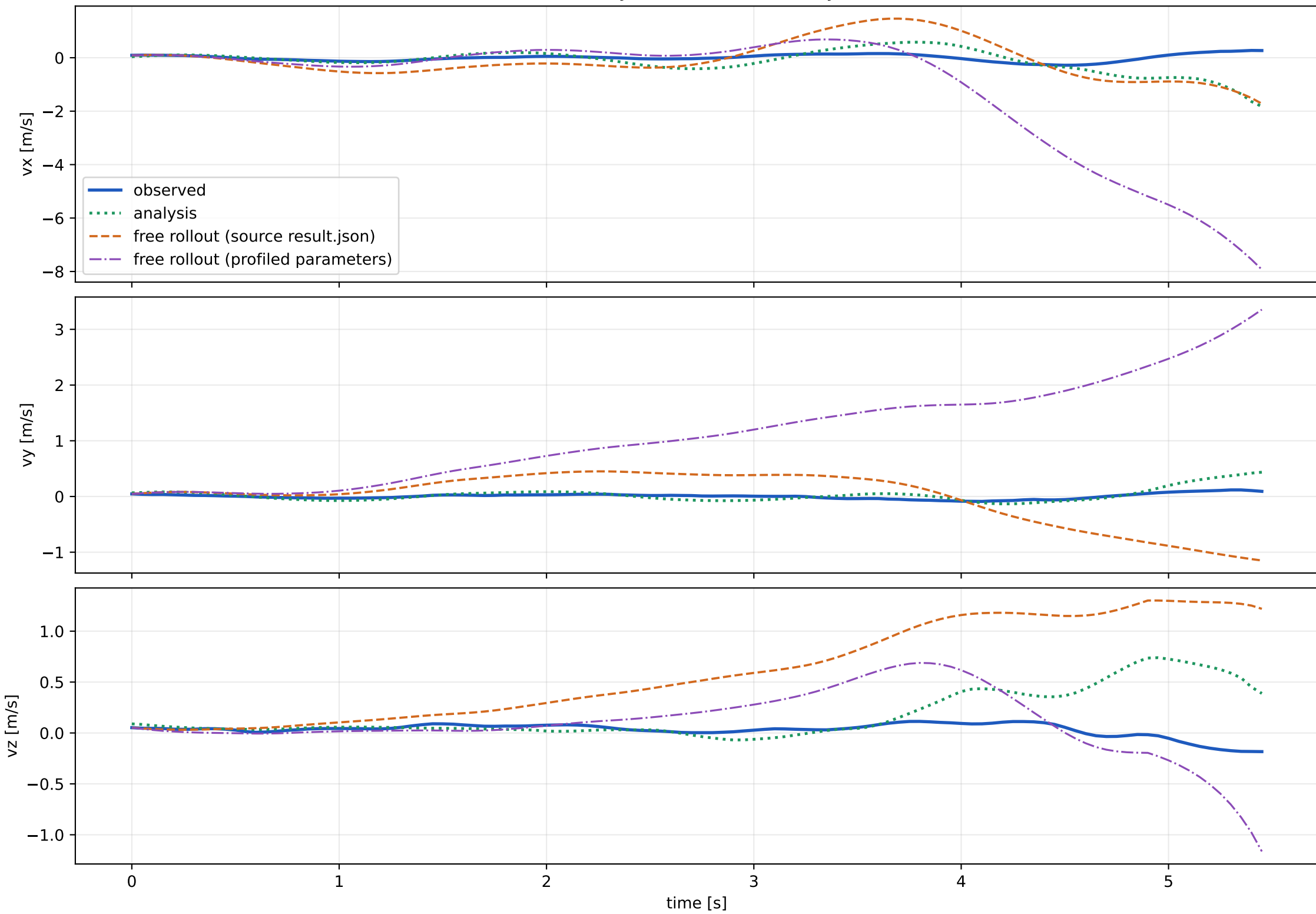
Velocity sensor linear velocity
