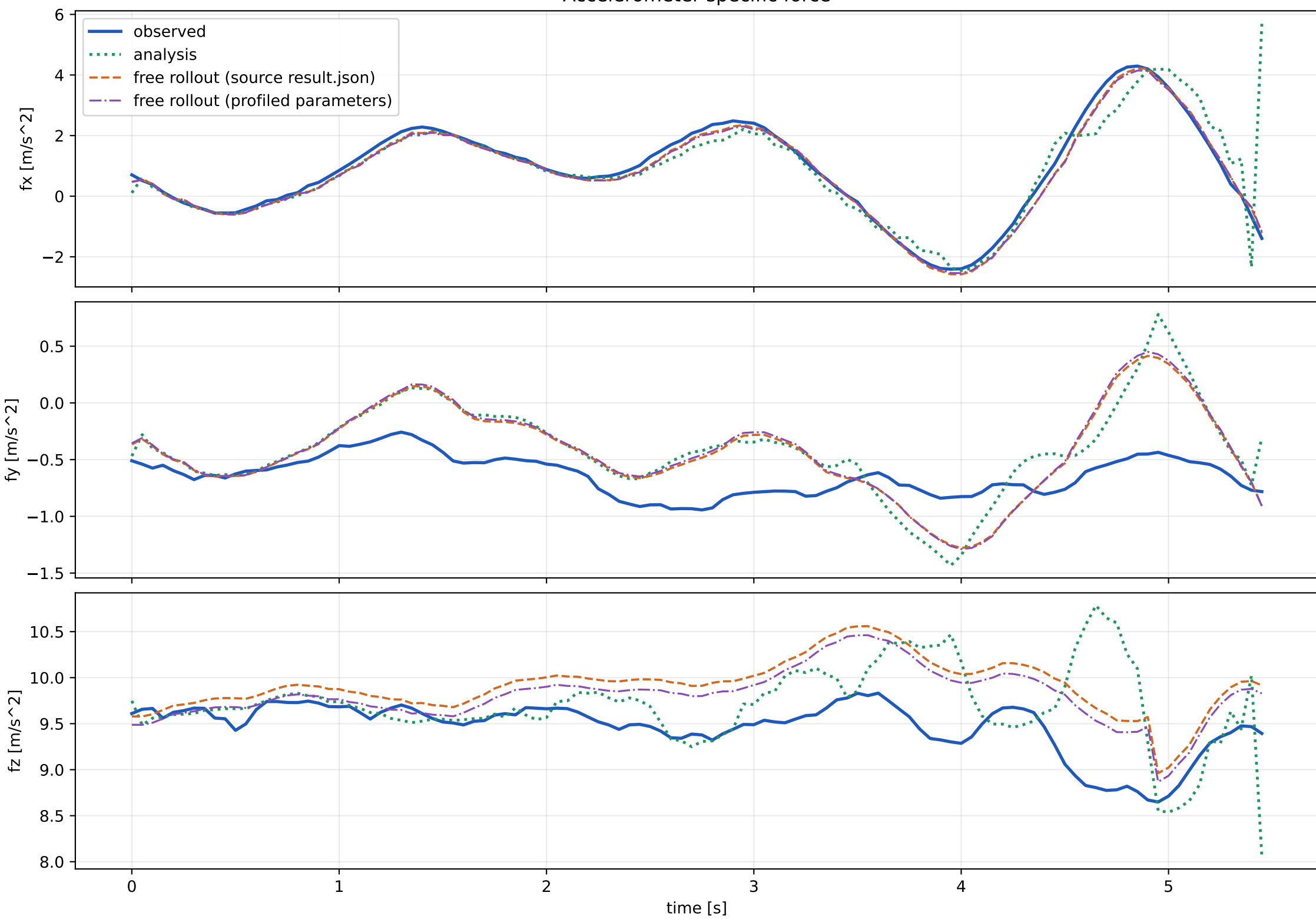
Accelerometer specific force
