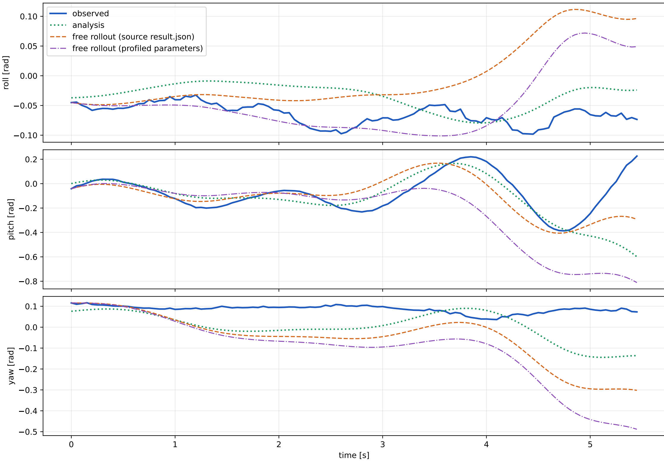
Sensor orientation
