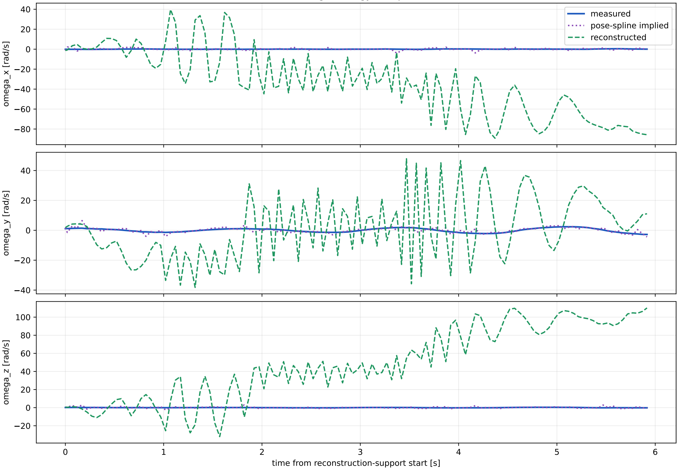
Diagnostic: gyroscope
