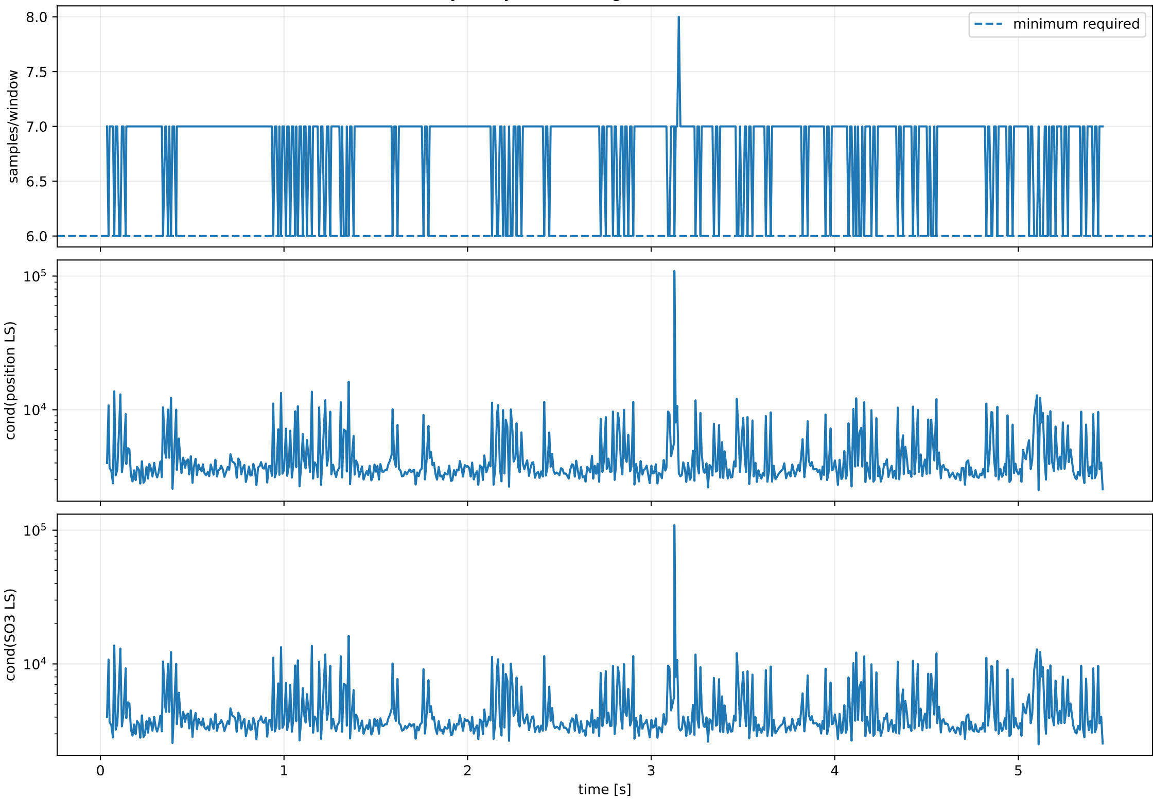
Savitzky-Golay window diagnostics; W=0.0533743s
