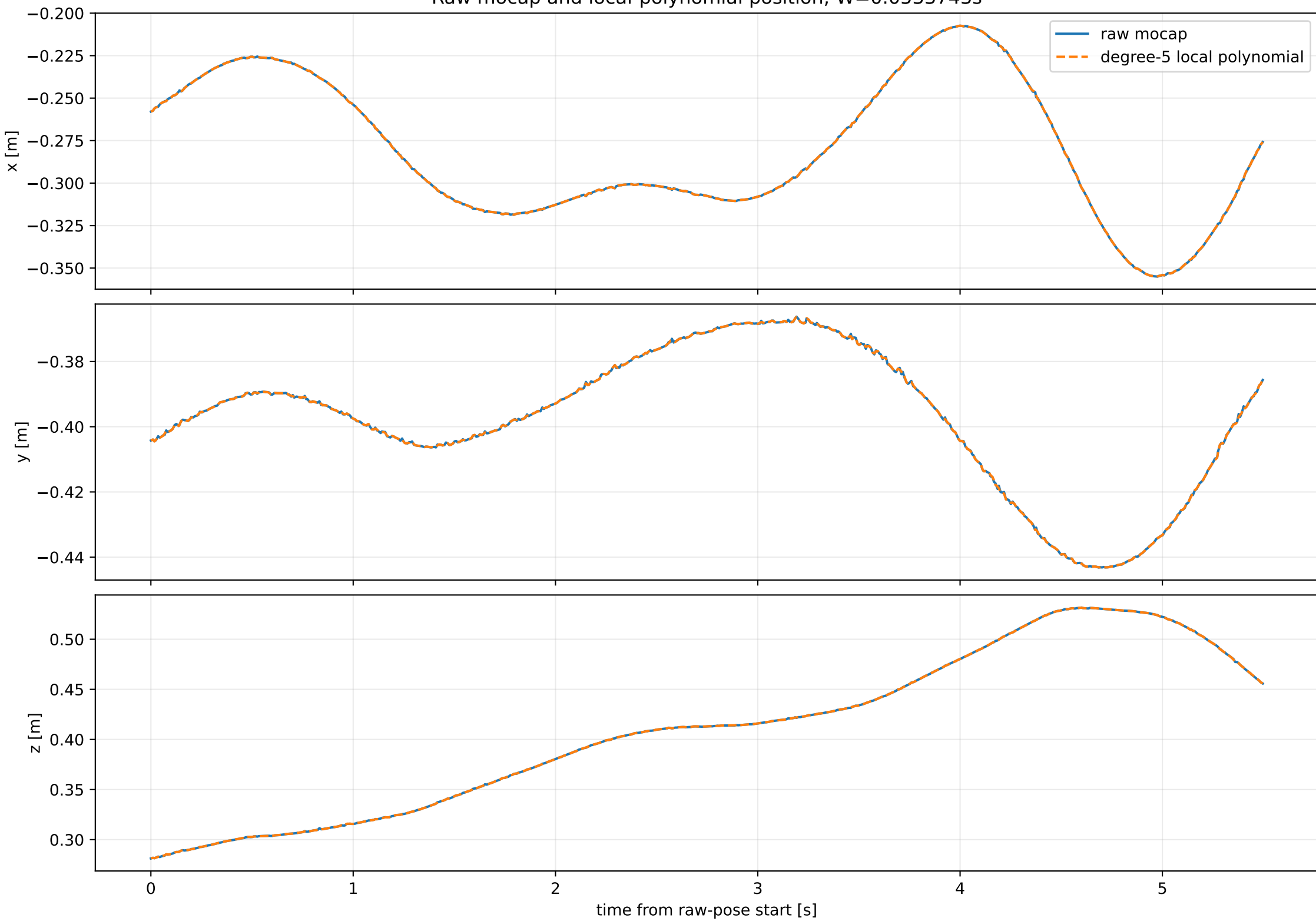
Raw mocap and local-polynomial position; W=0.0533743s
