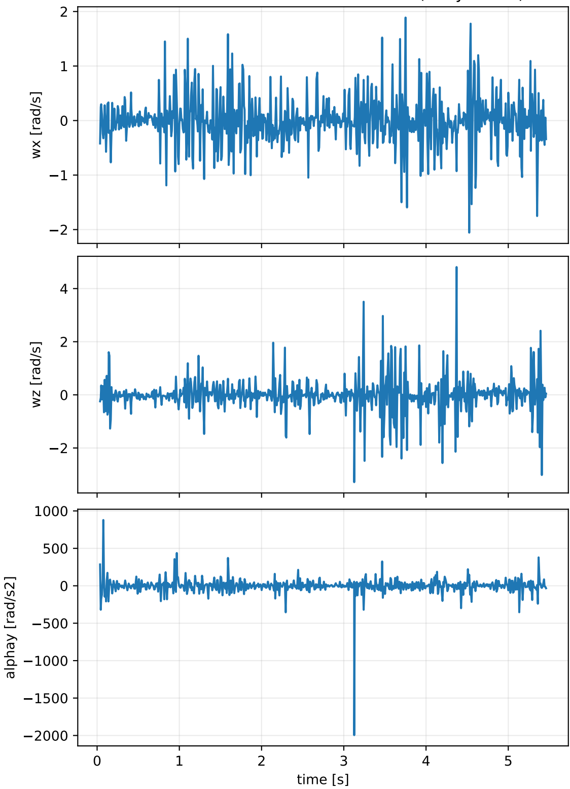
Geometric-SG rotational derivatives (body frame)
