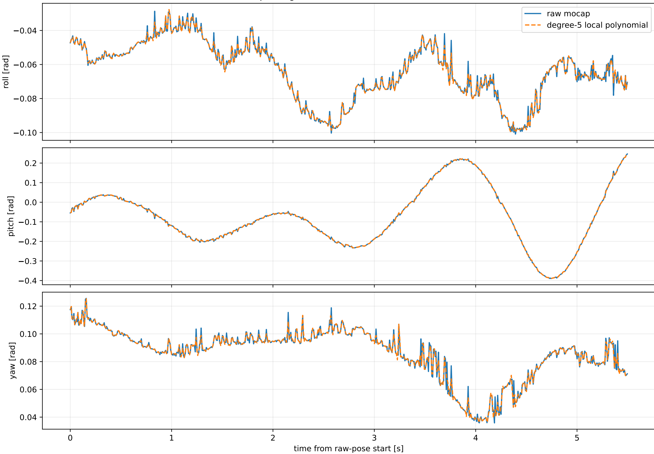
Raw mocap and geometric-SG orientation; W=0.0533743s
