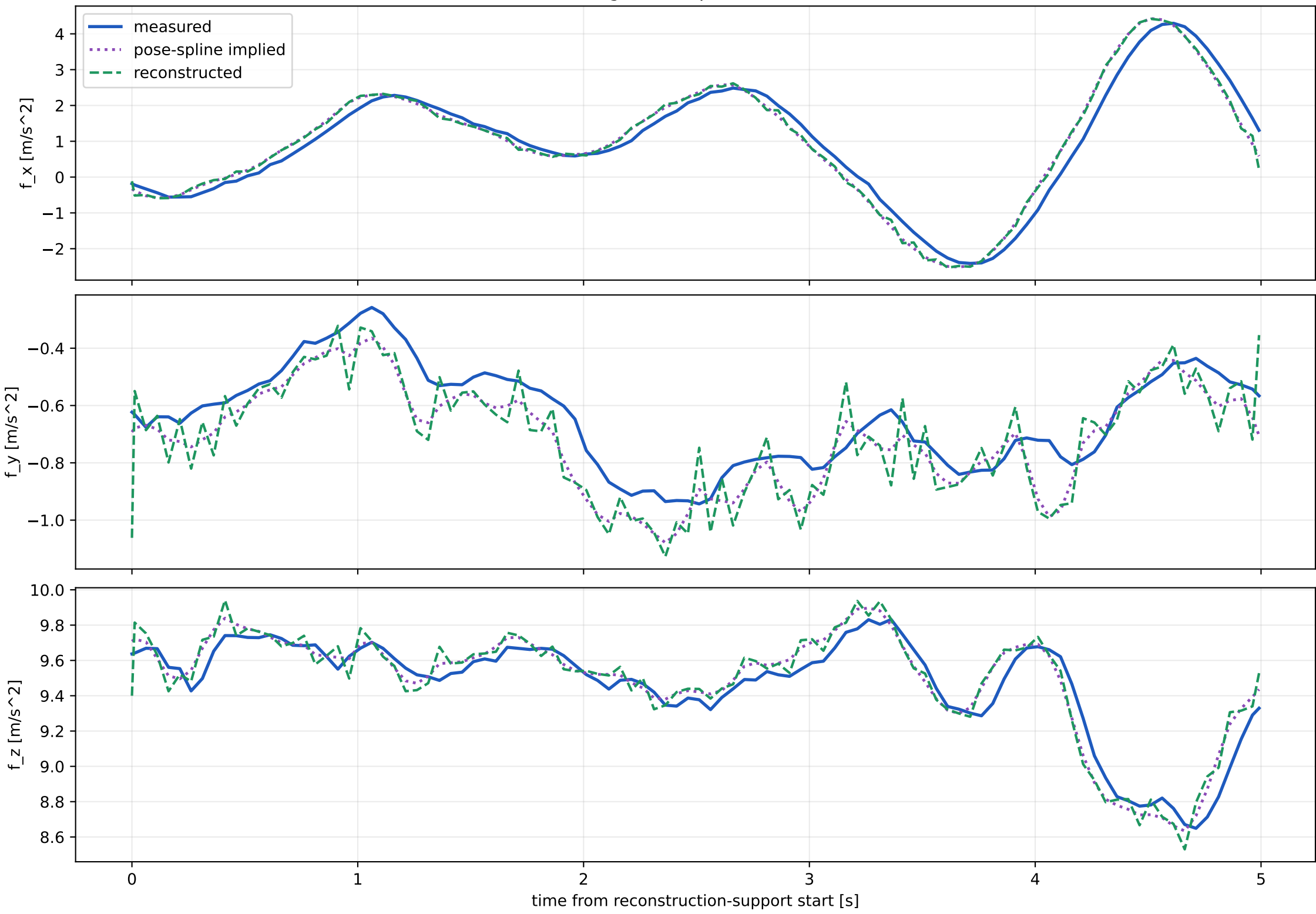
Diagnostic: specific force
