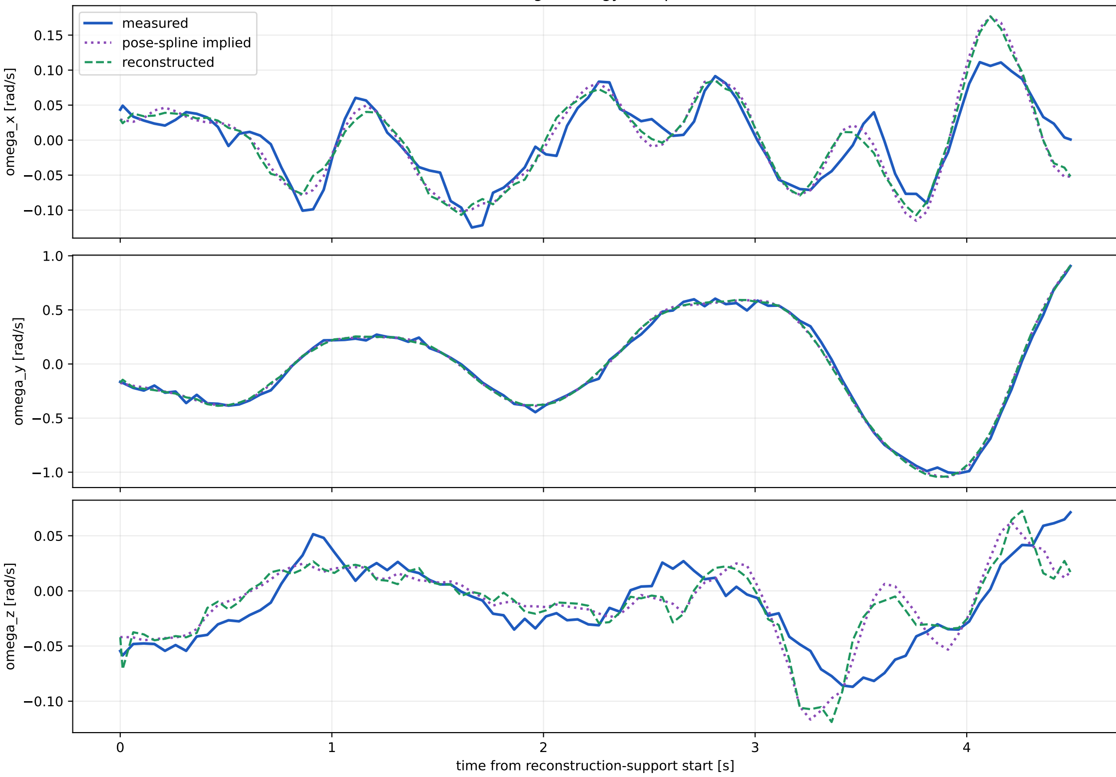
Diagnostic: gyroscope
