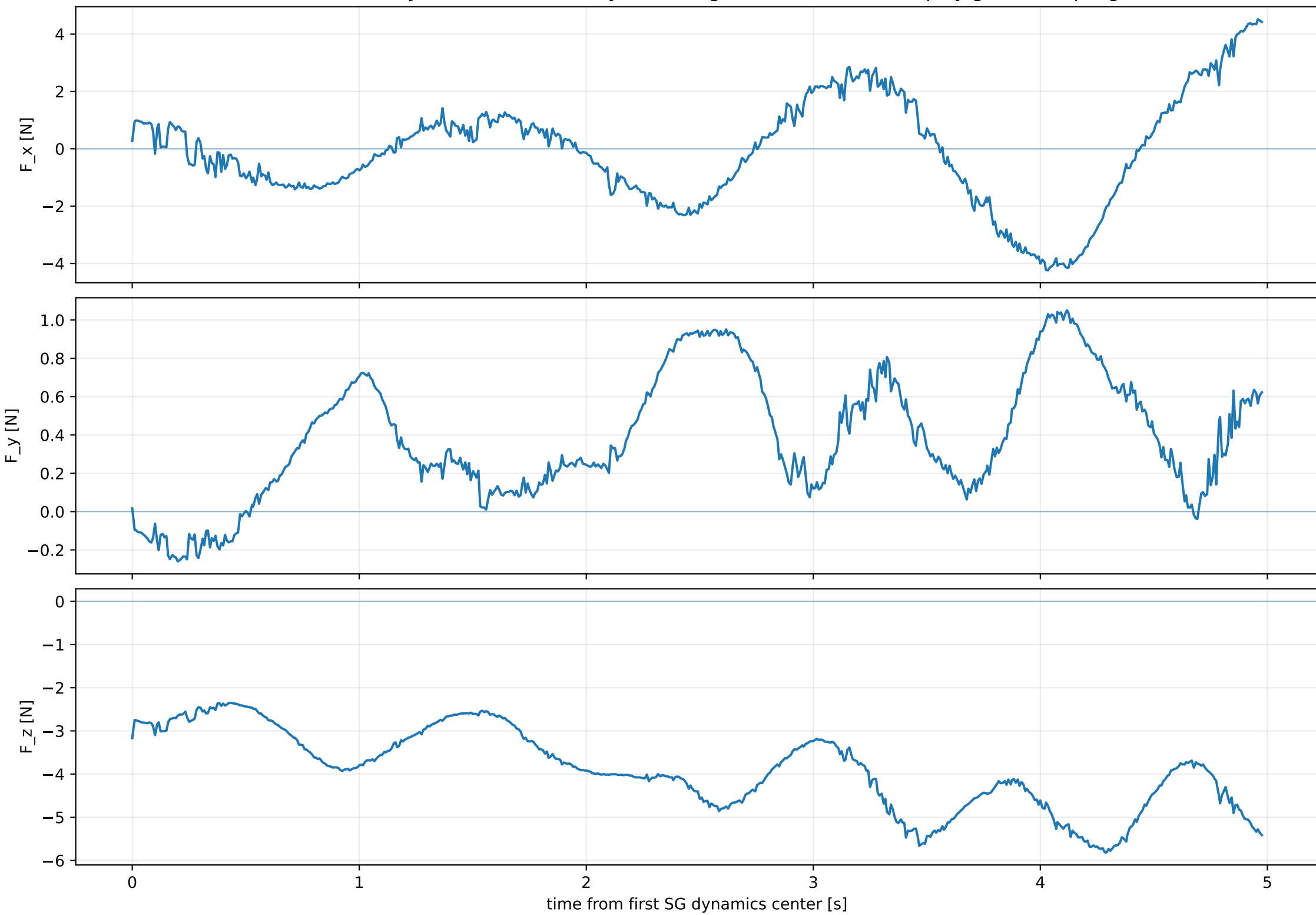
Raw inverse-dynamics residual body force; degree-5 SG W=1s; no replay-grid resampling
