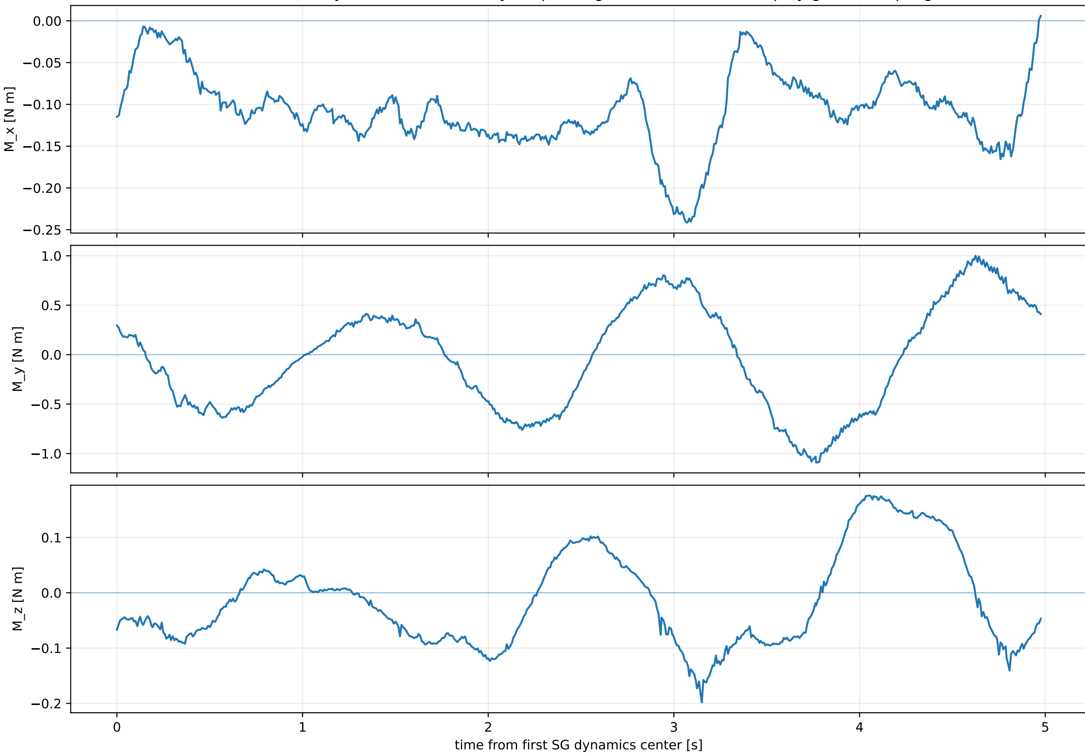
Raw inverse-dynamics residual body torque; degree-5 SG W=1s; no replay-grid resampling
