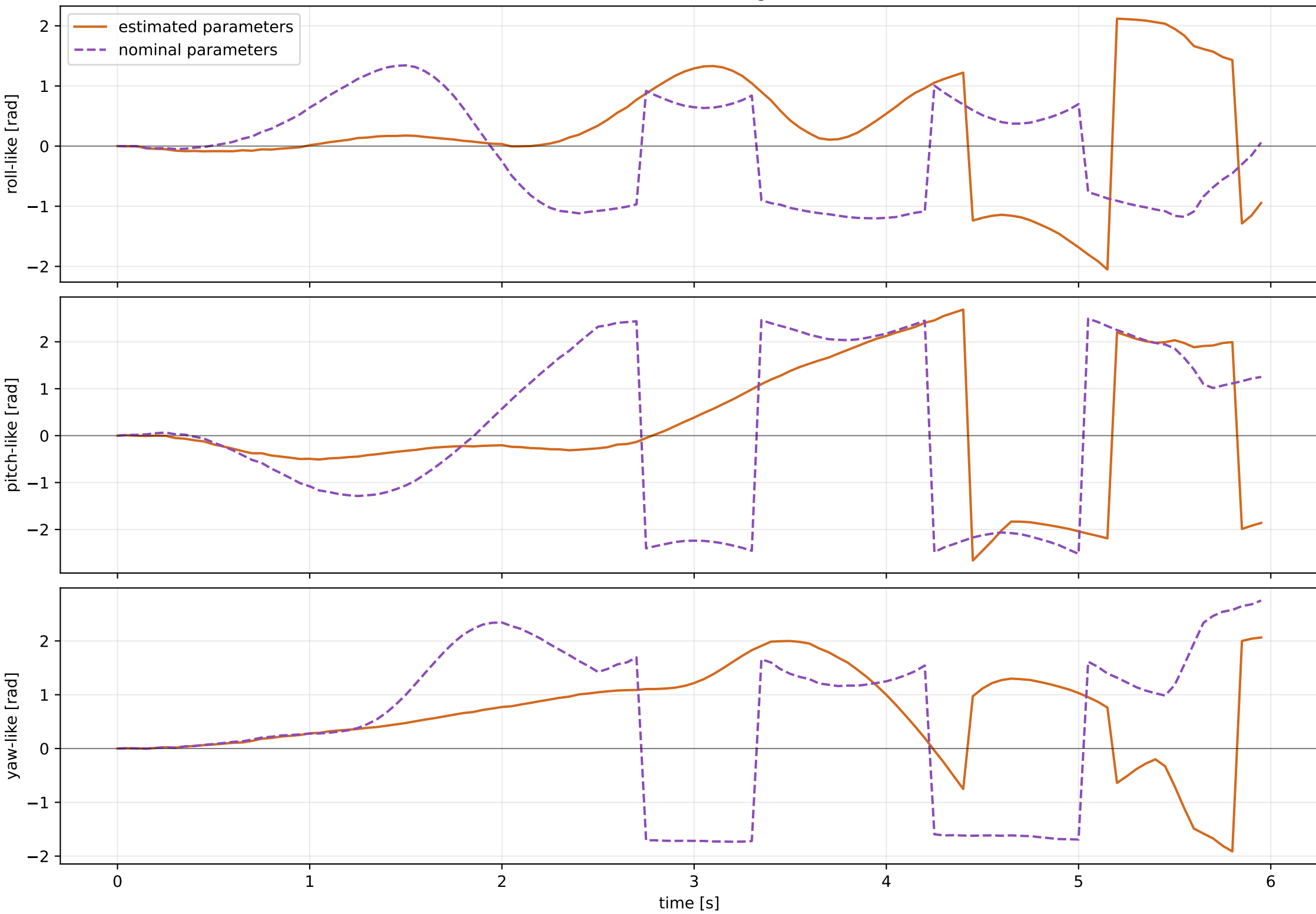
Sensor orientation log error
