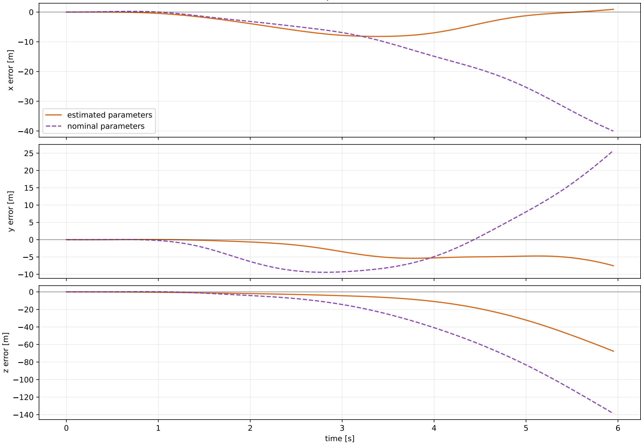
Sensor position error
