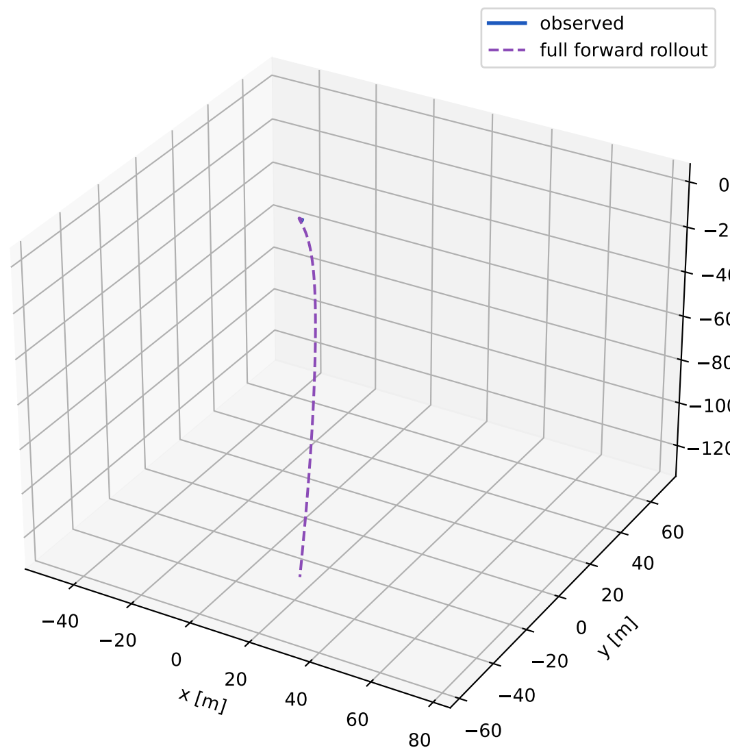
Nominal parameters: full forward rollout
