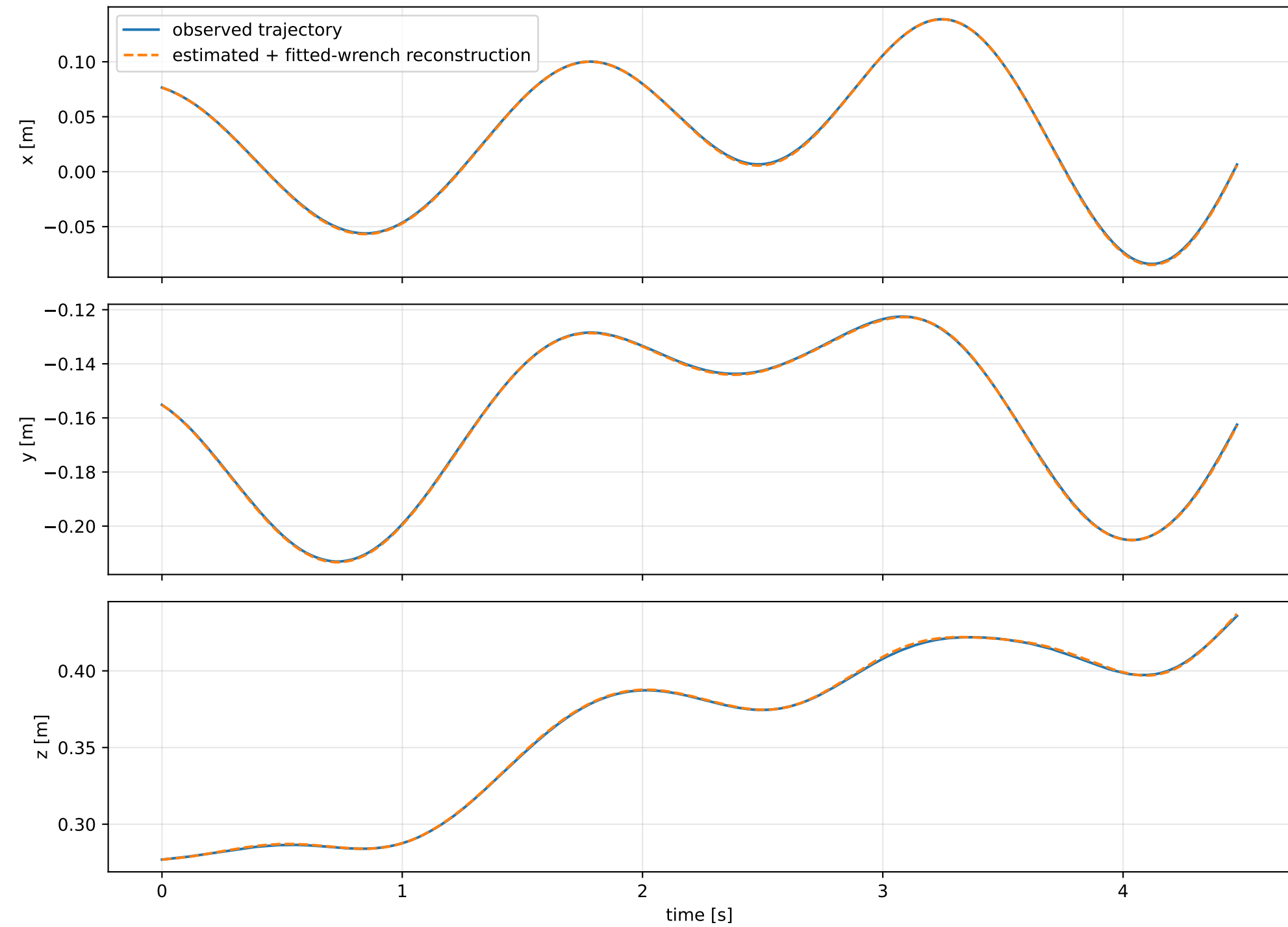
sweep_sg_window_covariance__002: trajectory
