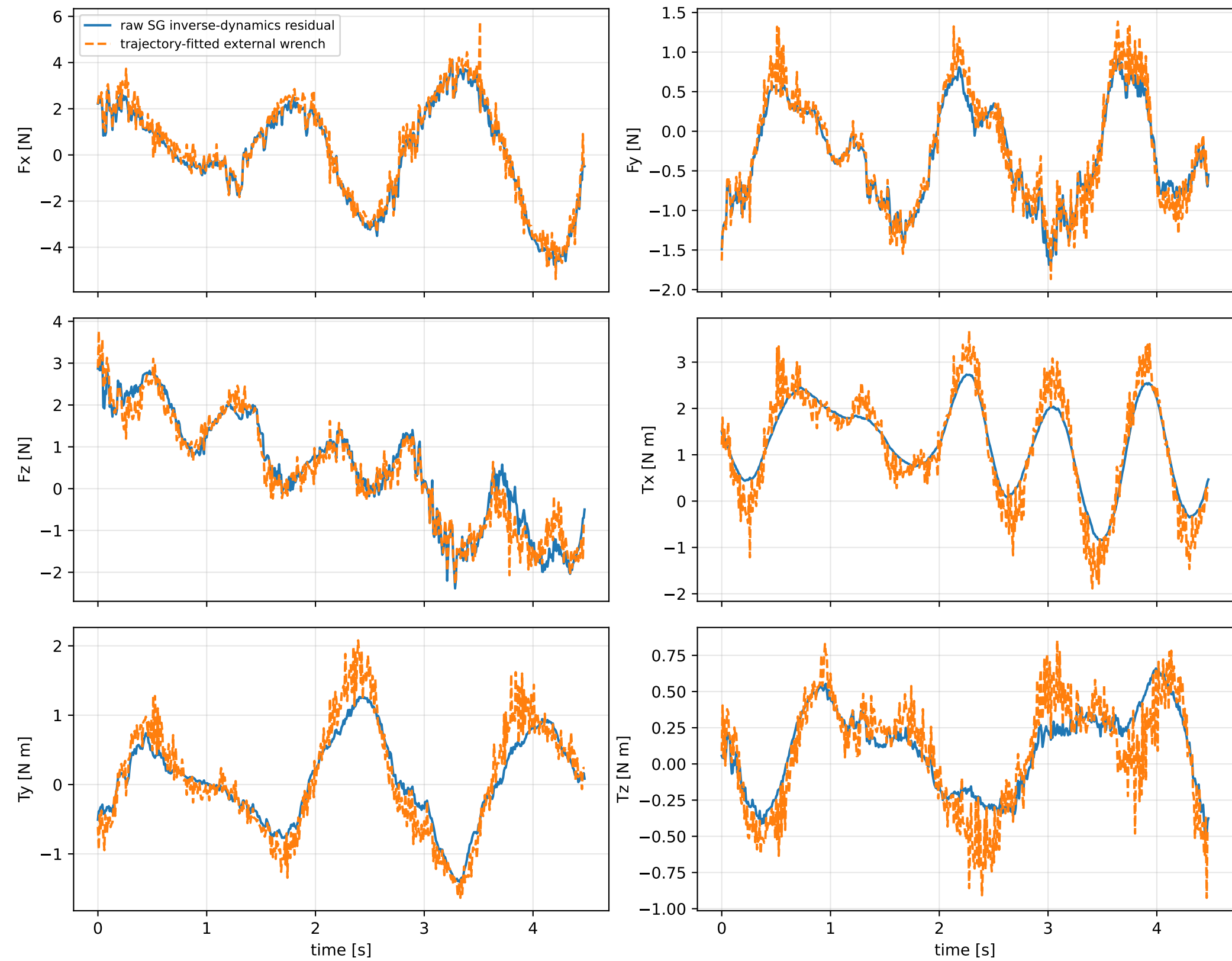
sweep_sg_window_covariance_002: residual wrench
