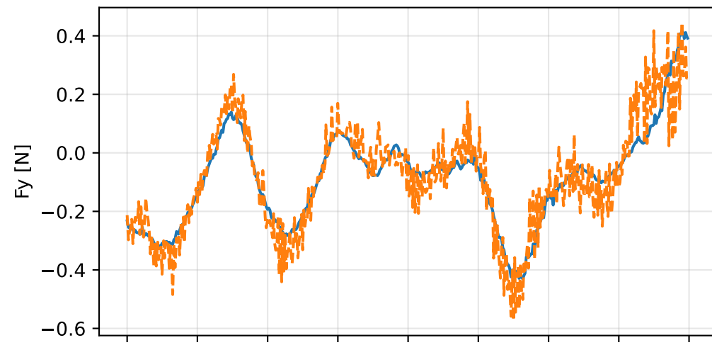
sweep_sg_window_covariance_003: residual wrench
