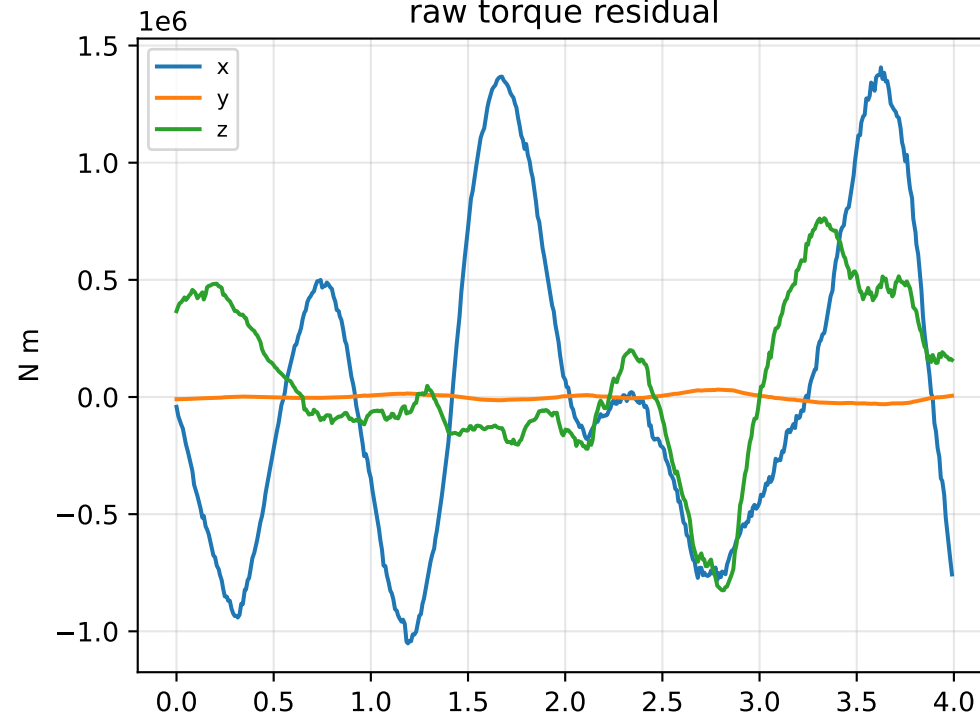
raw torque residual
