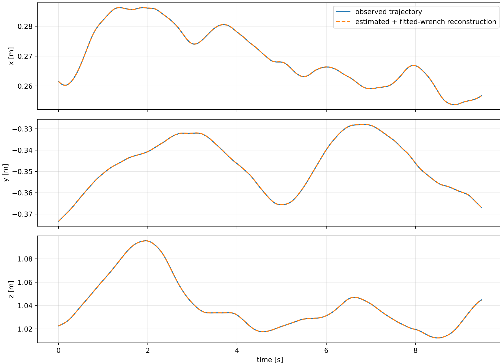
cov_identity: trajectory
