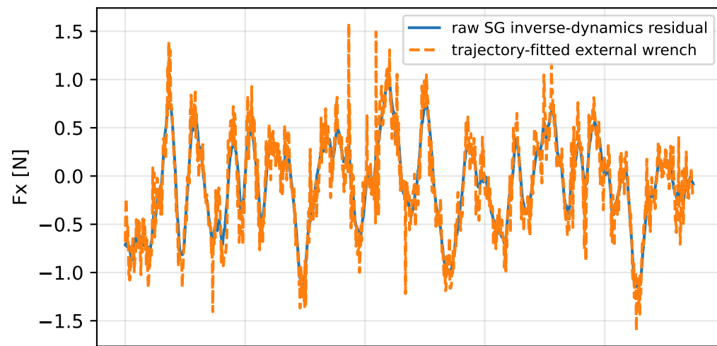
default_full_covariance: residual wrench
