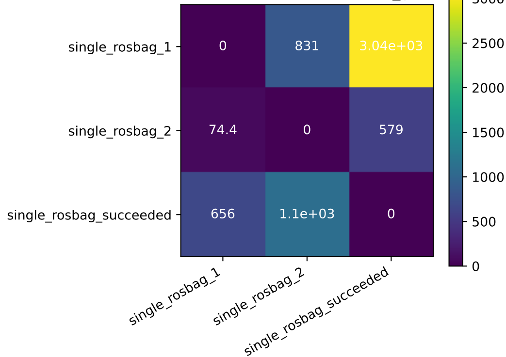
cross-evaluation Delta L ij
