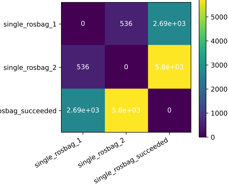
pairwise quotient distance: SG overlap
