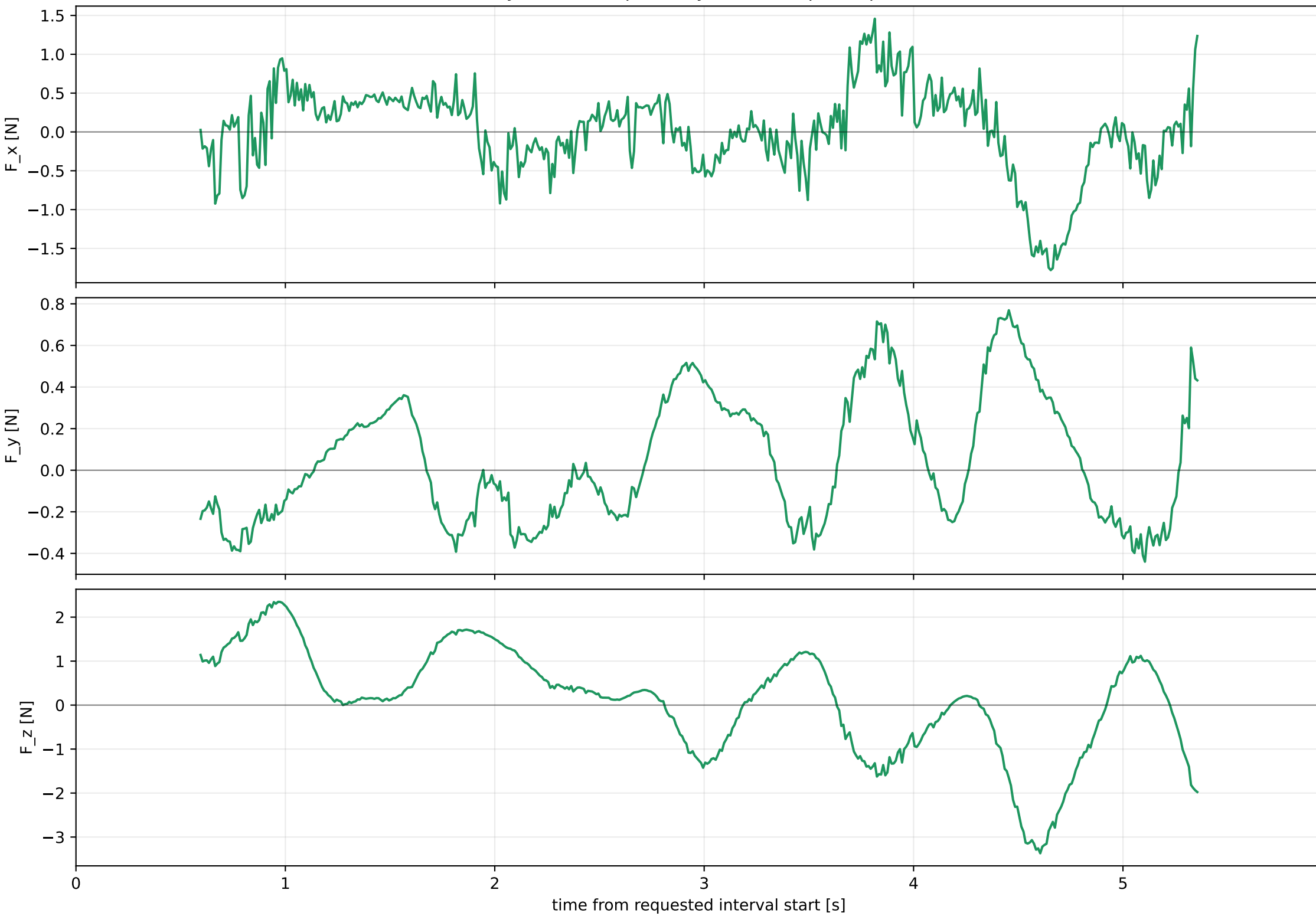
Inferred external body force = required by observed-pose spline - modeled wrench
