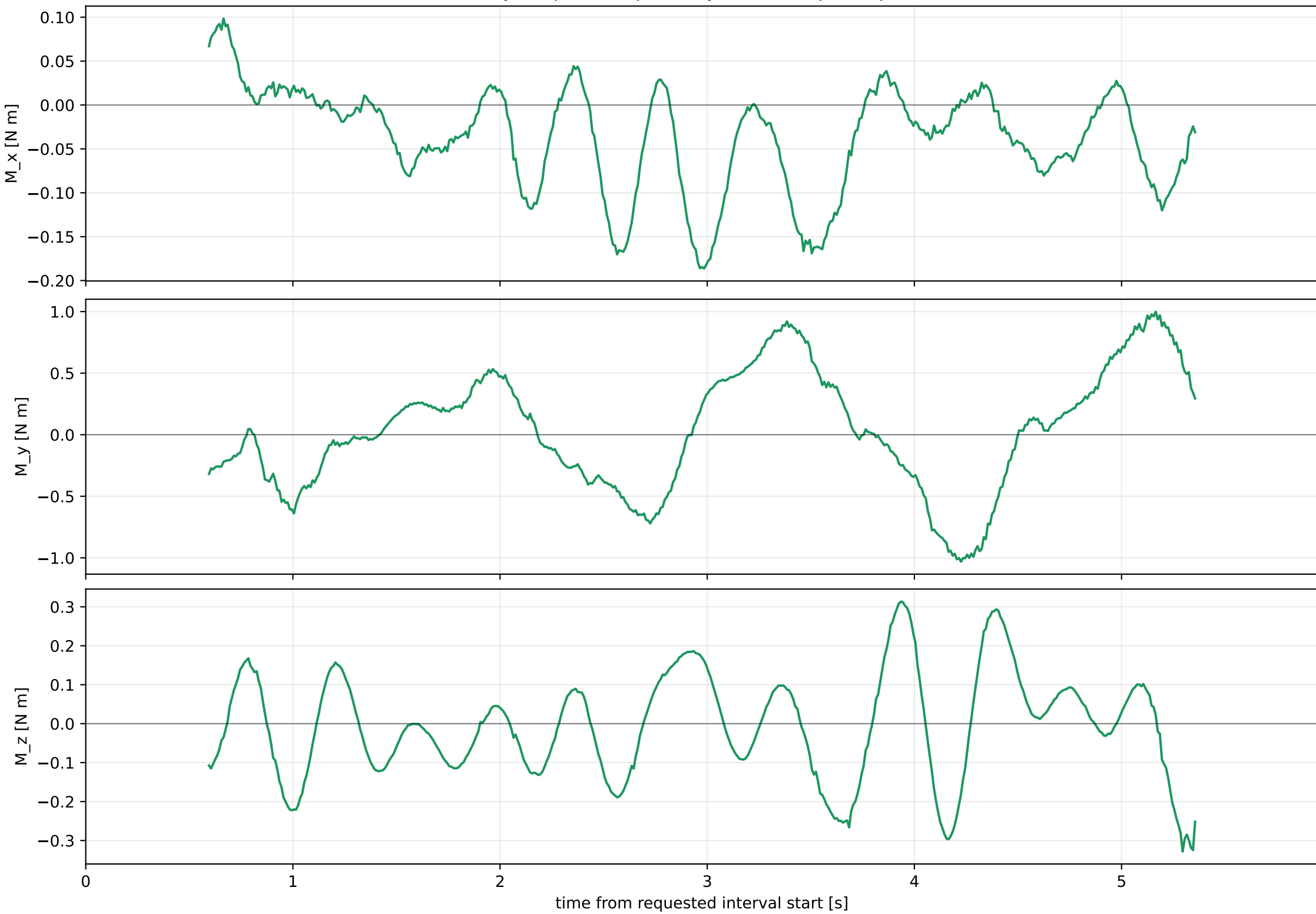
Inferred external body torque = required by observed-pose spline - modeled wrench
