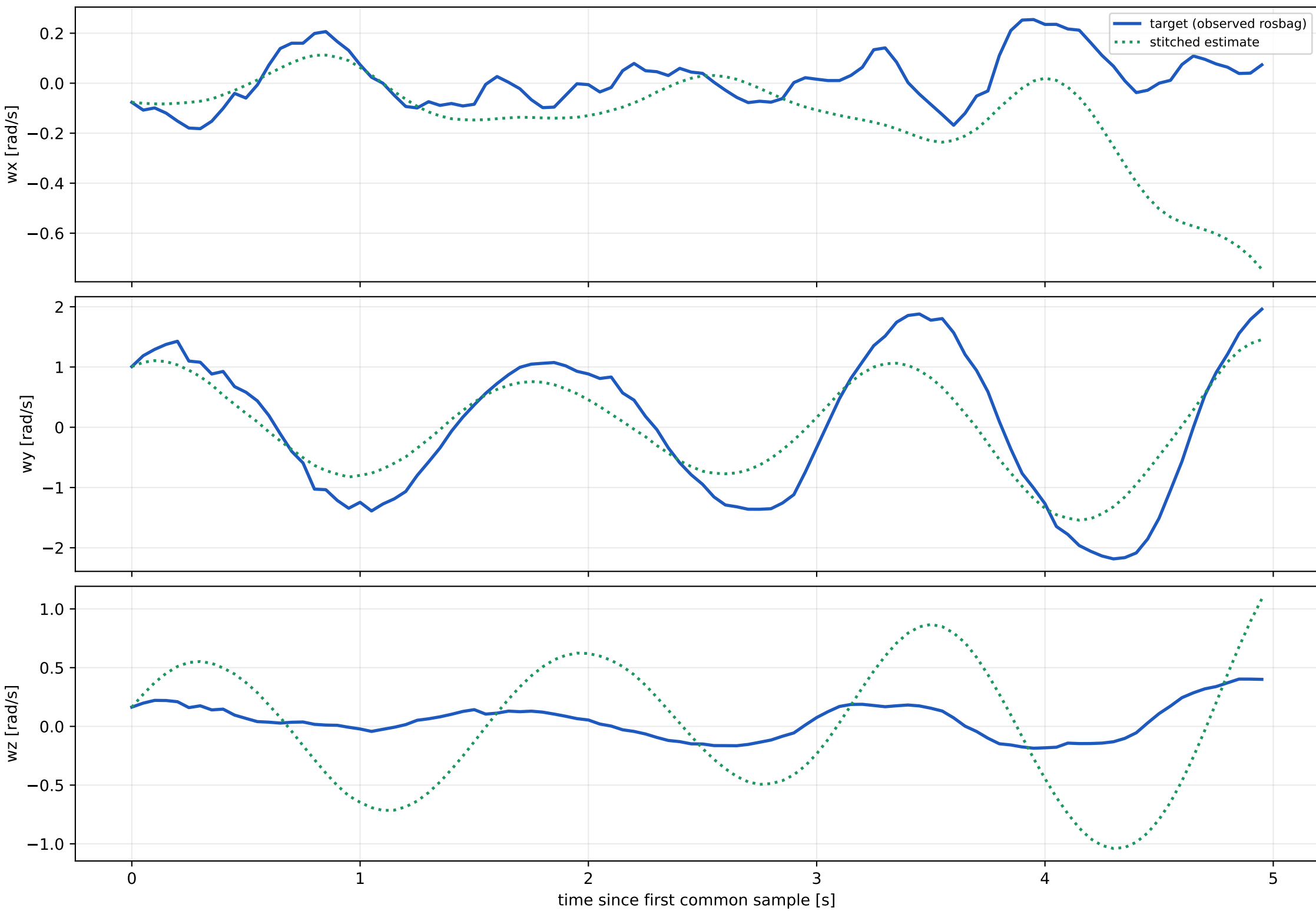
IMU angular velocity (diagnostic; excluded from fit)
