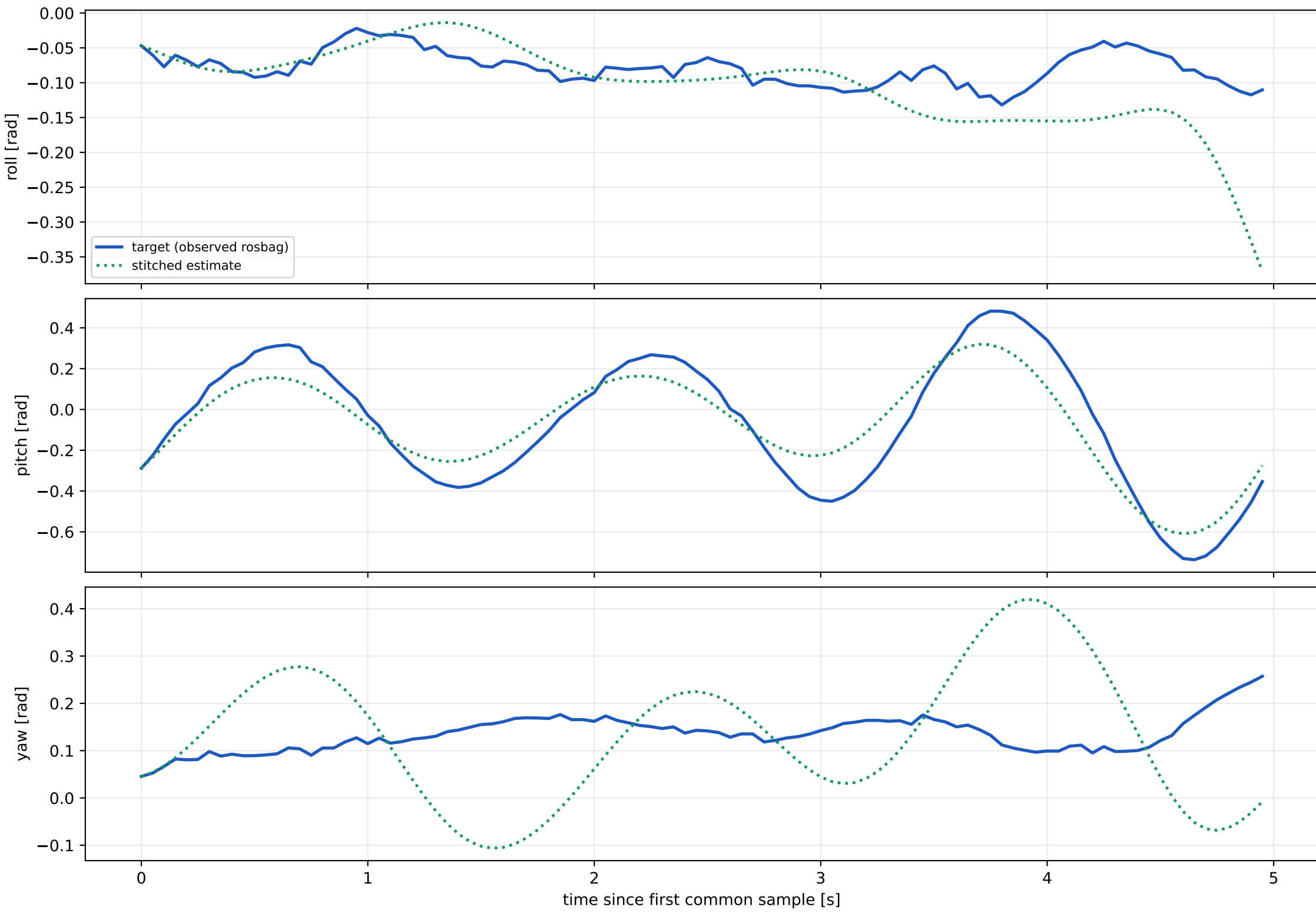
Sensor orientation (display only; fit uses SO(3) log)
