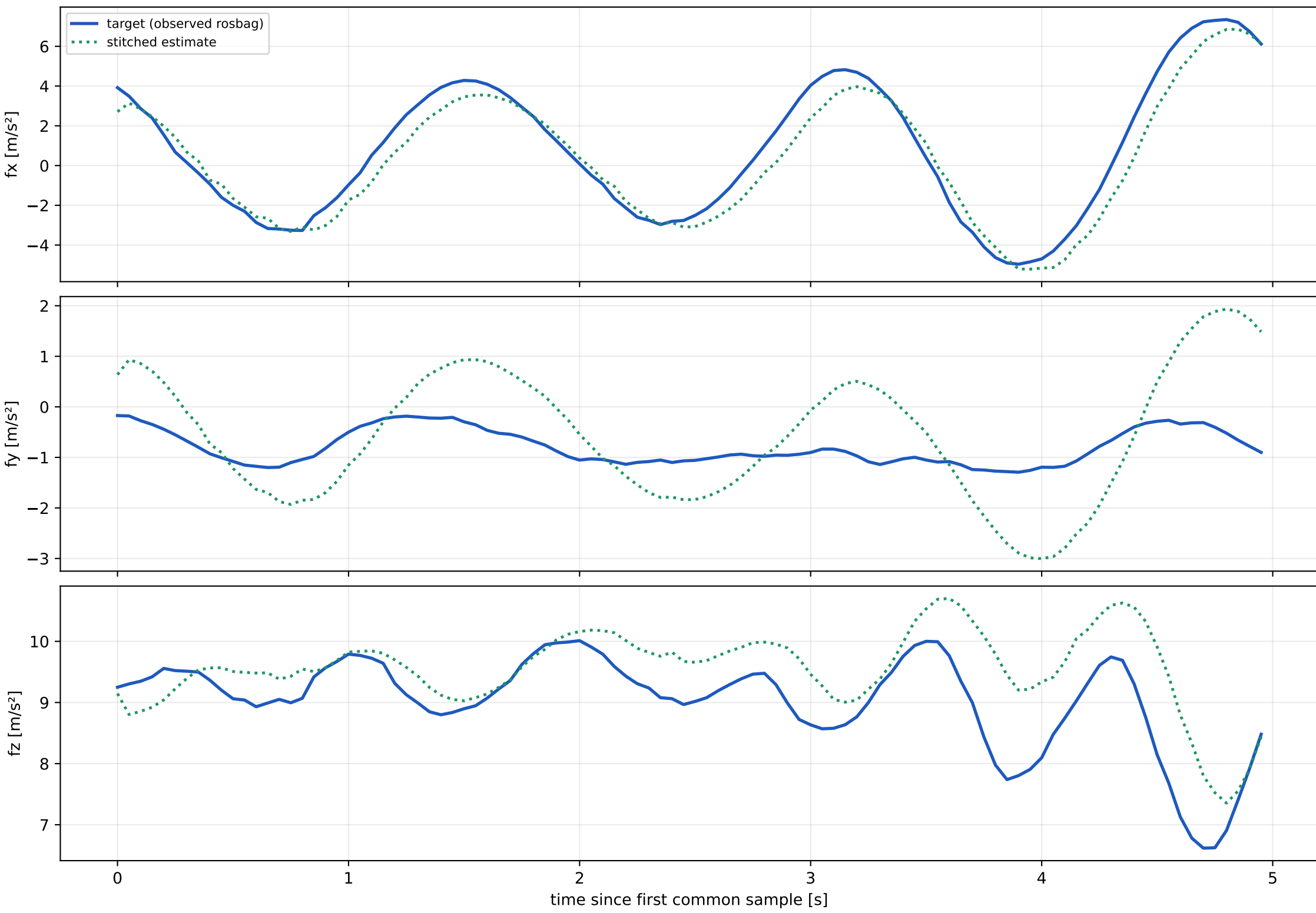
IMU specific force (diagnostic; excluded from fit)
