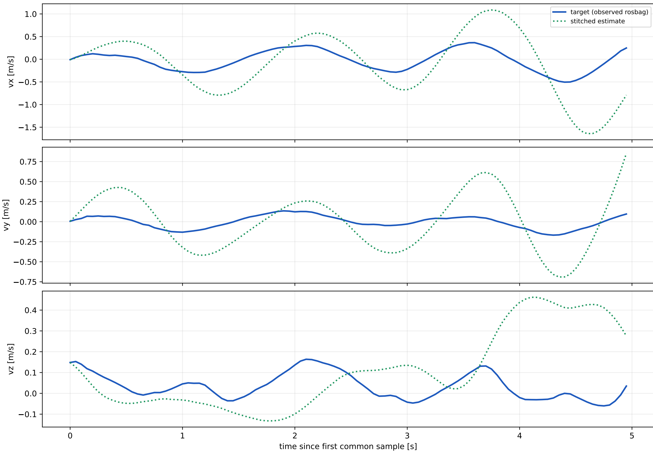
World-frame sensor velocity (diagnostic; excluded from fit)
