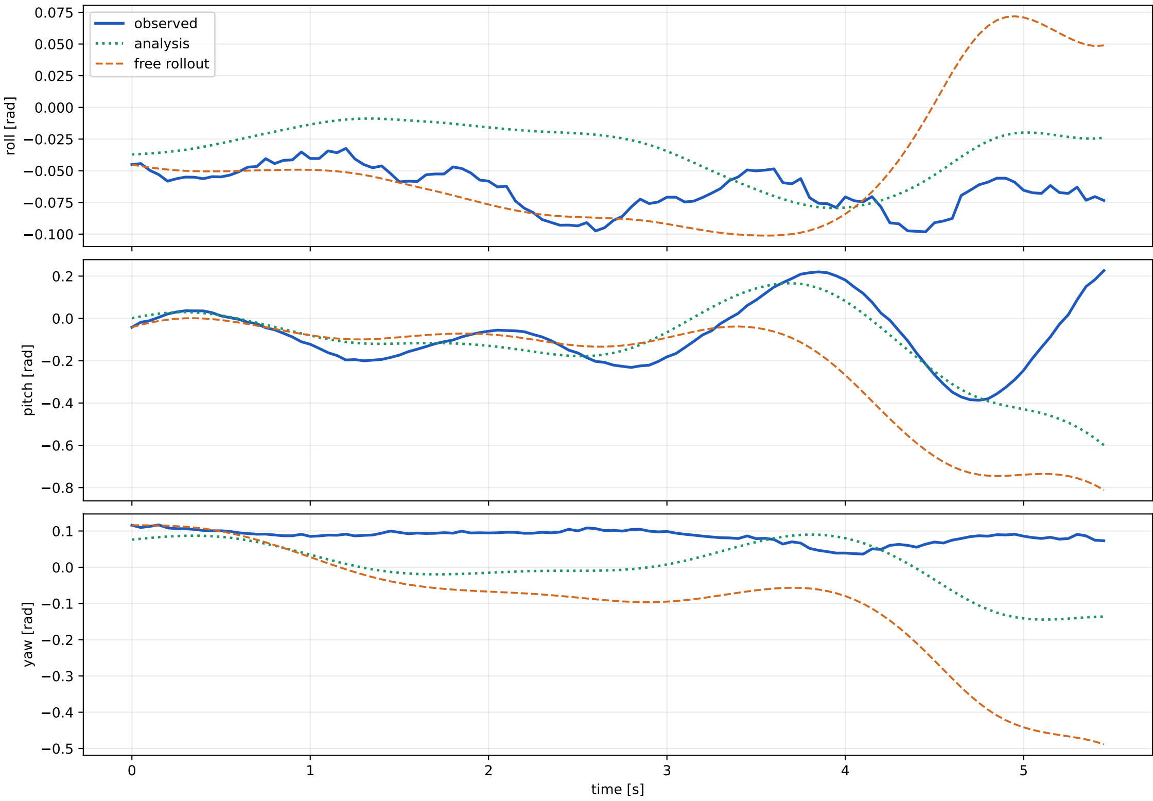
Sensor orientation
