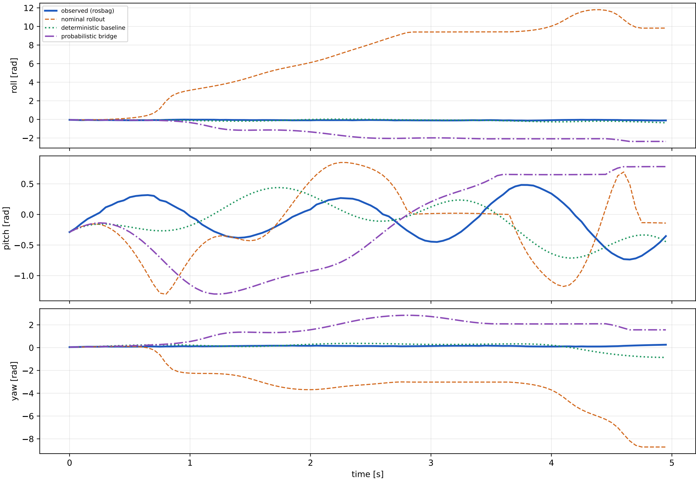
Sensor orientation RPY
