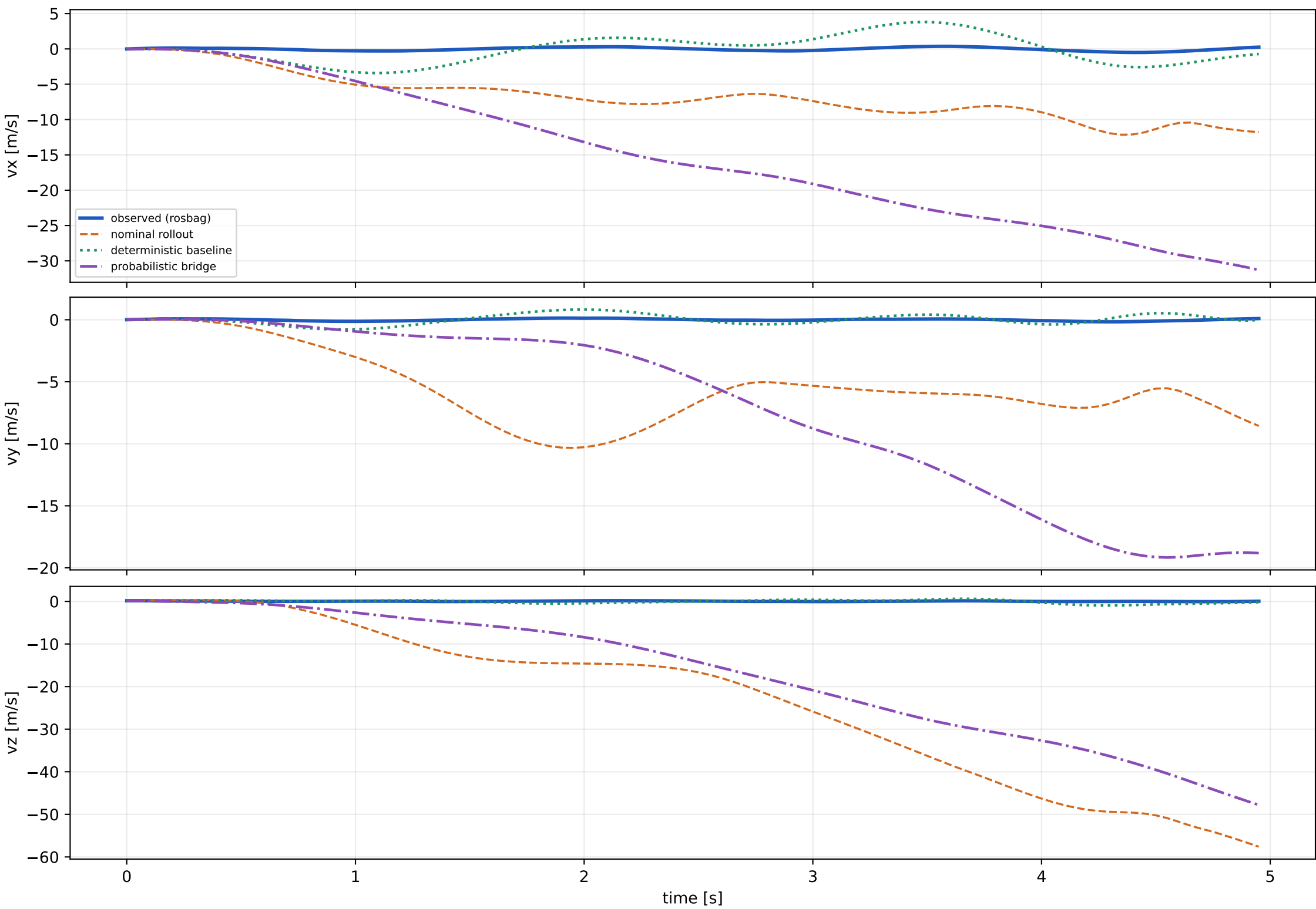
Sensor velocity
