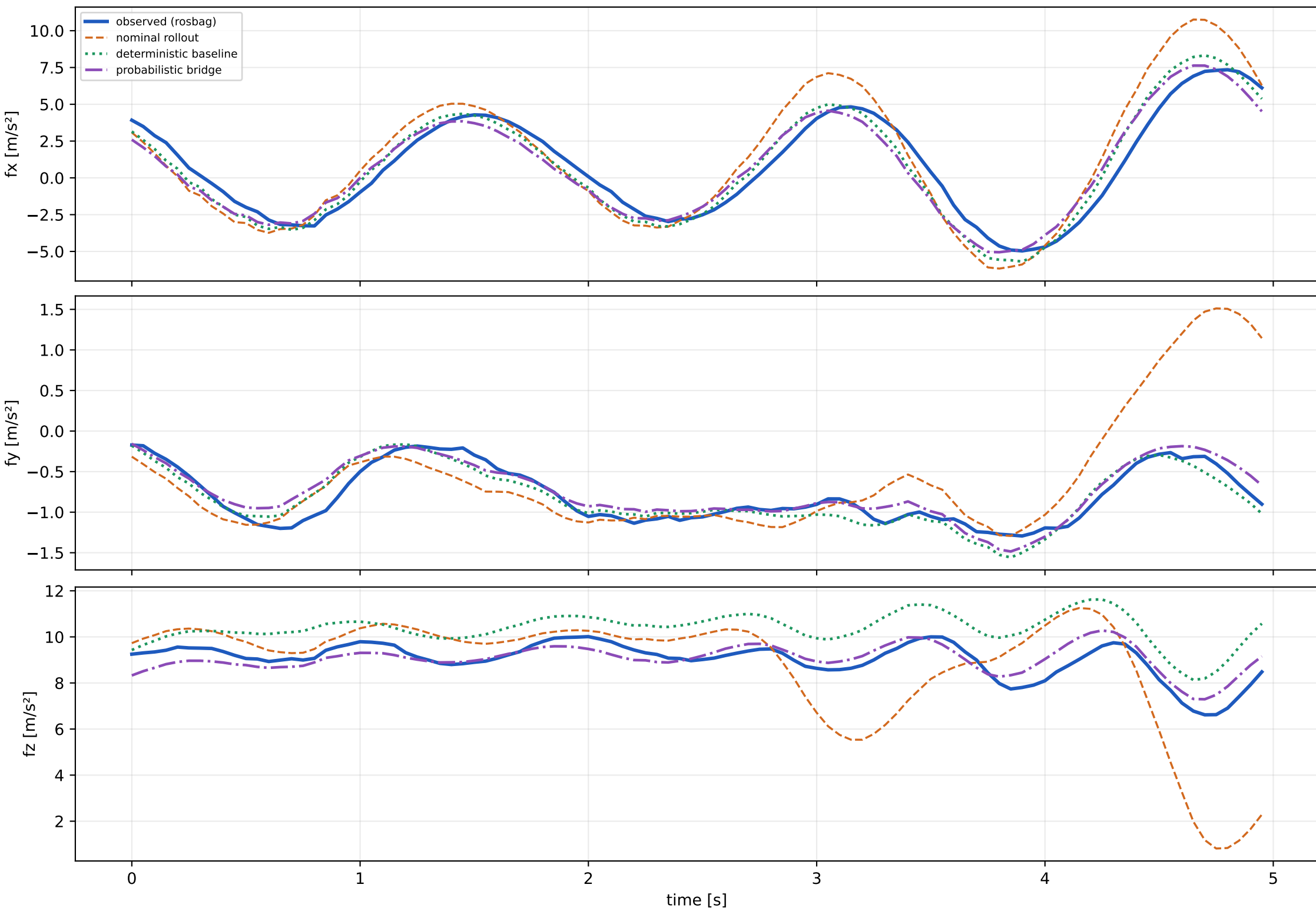
IMU specific force
