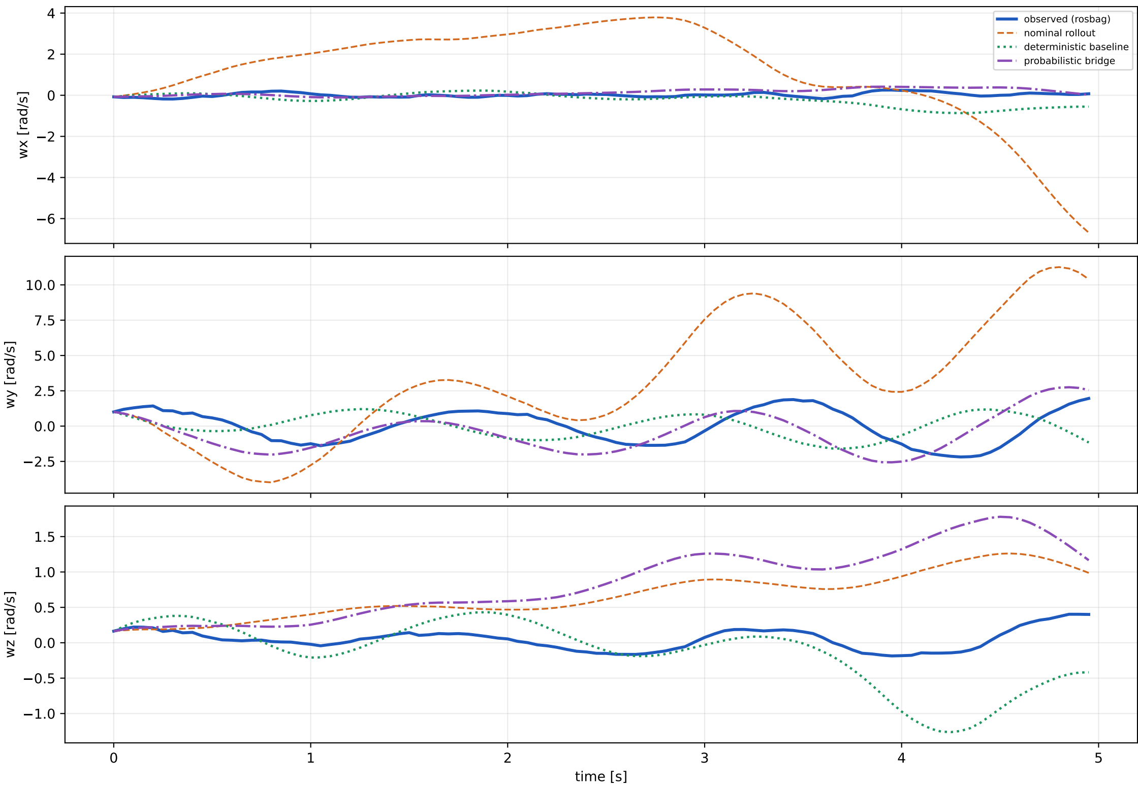
IMU angular velocity
