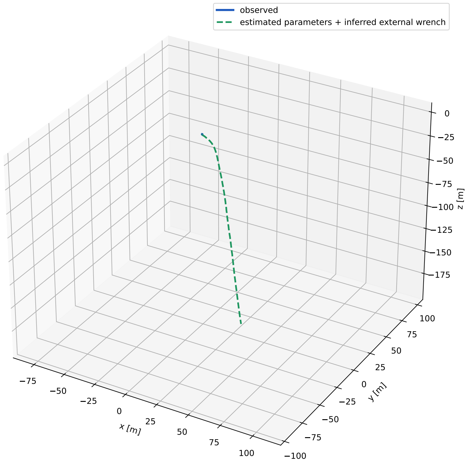
Observed and reconstructed 3D trajectory
