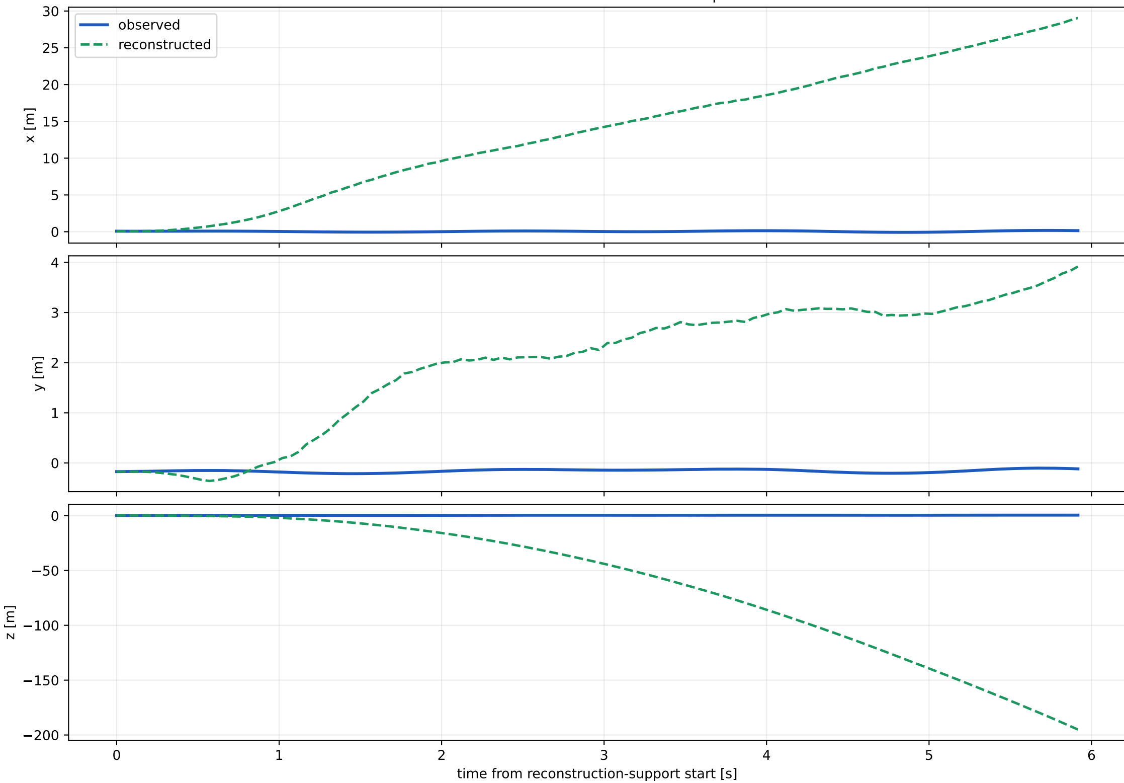
Observed and reconstructed sensor position
