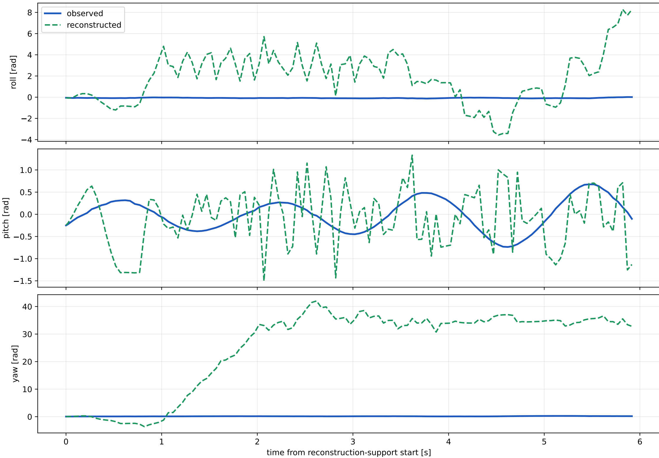
Observed and reconstructed sensor orientation
