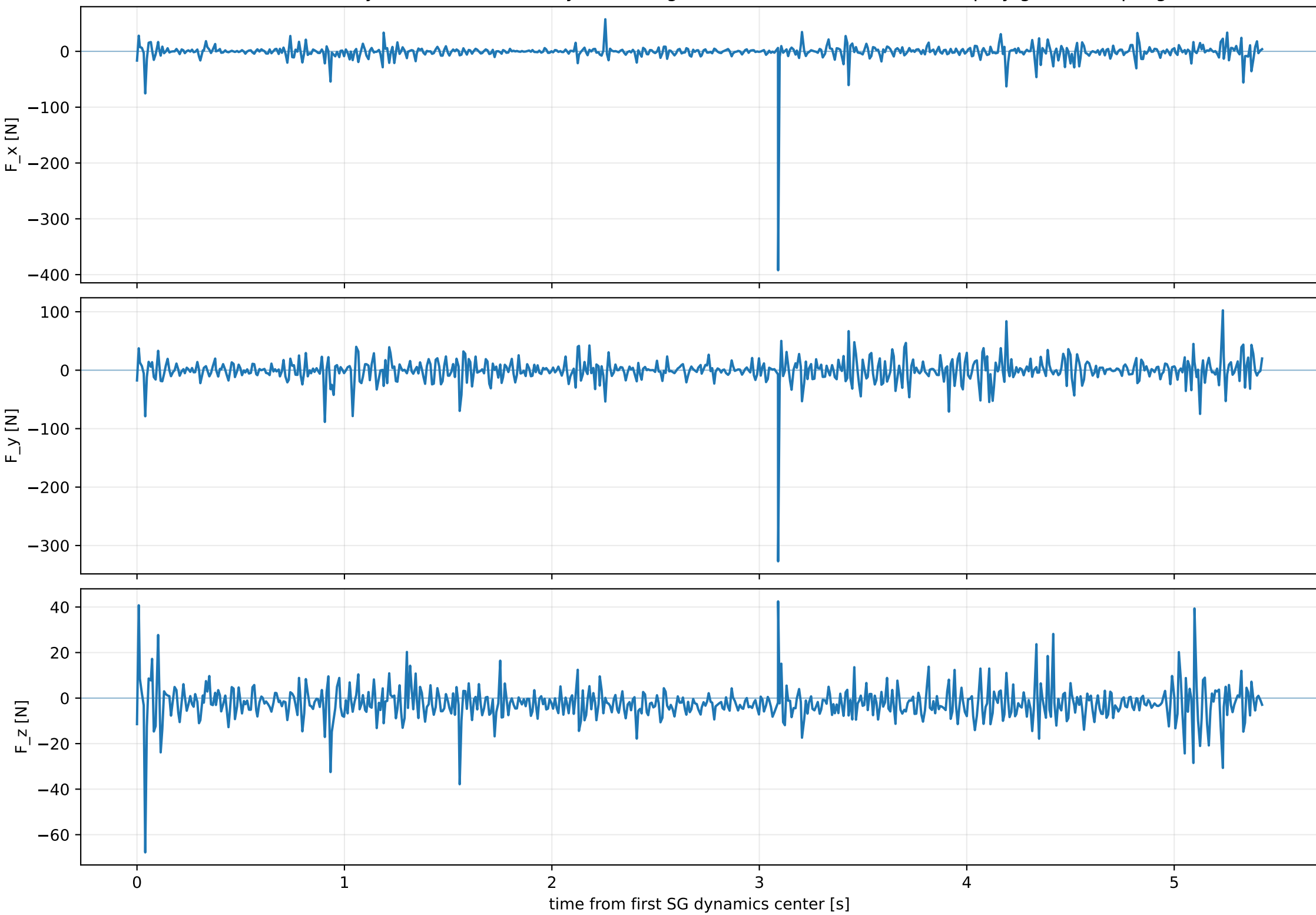
Raw inverse-dynamics residual body force; degree-5 SG W=0.0533743 s; no replay-grid resampling
