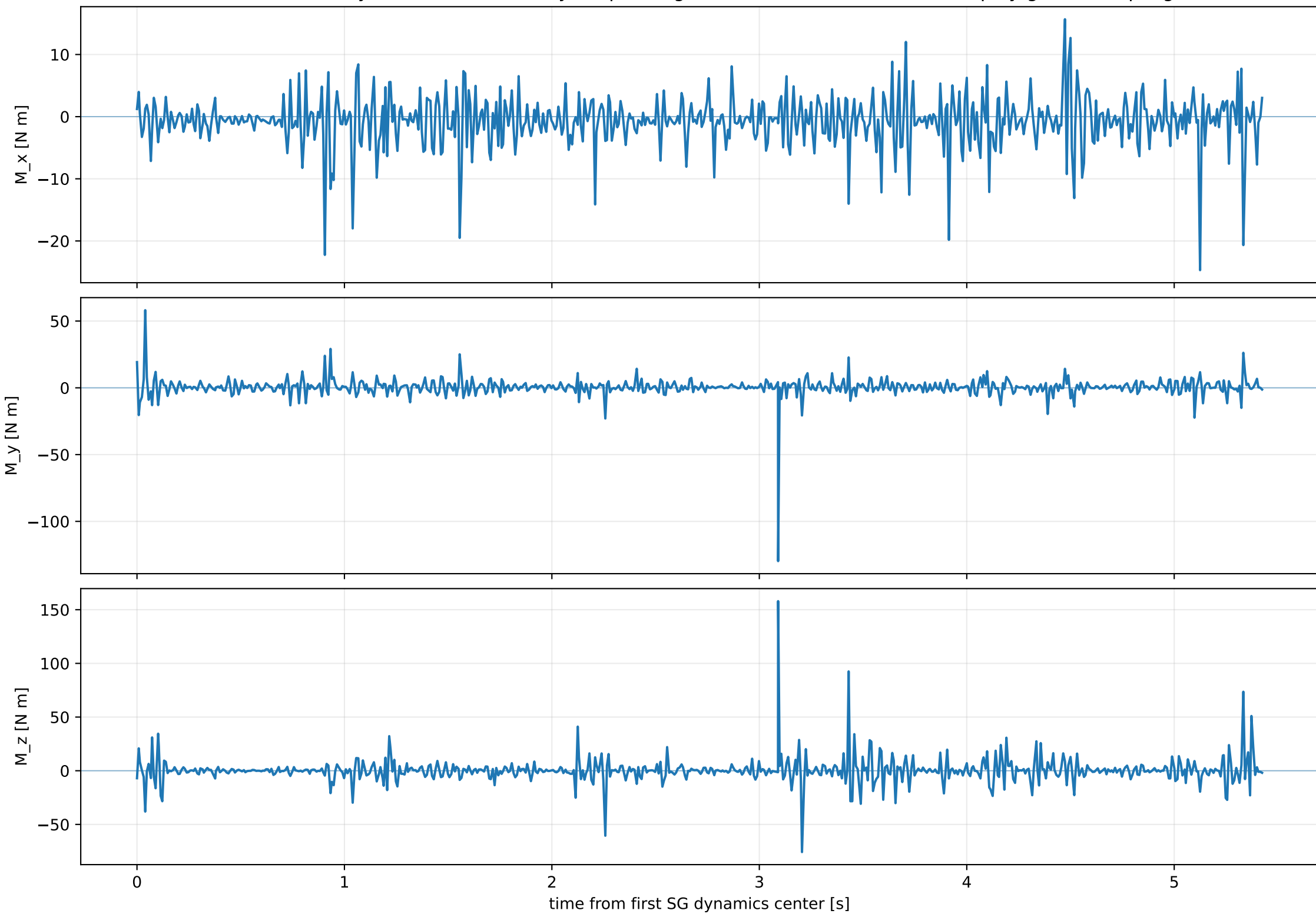
Raw inverse-dynamics residual body torque; degree-5 SG W=0.0533743s; no replay-grid resampling
