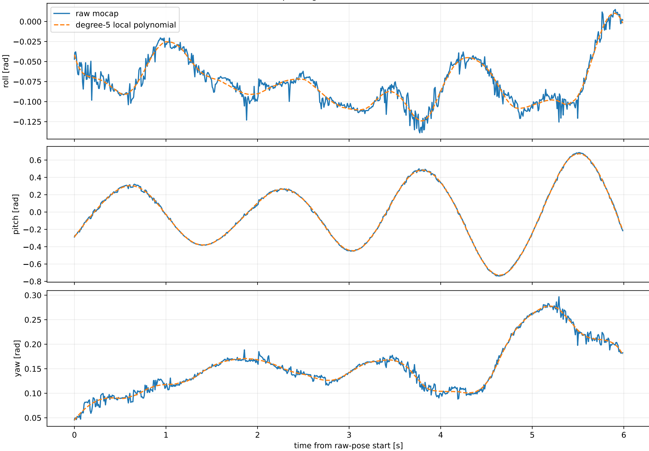
Raw mocap and geometric-SG orientation; W=1s
