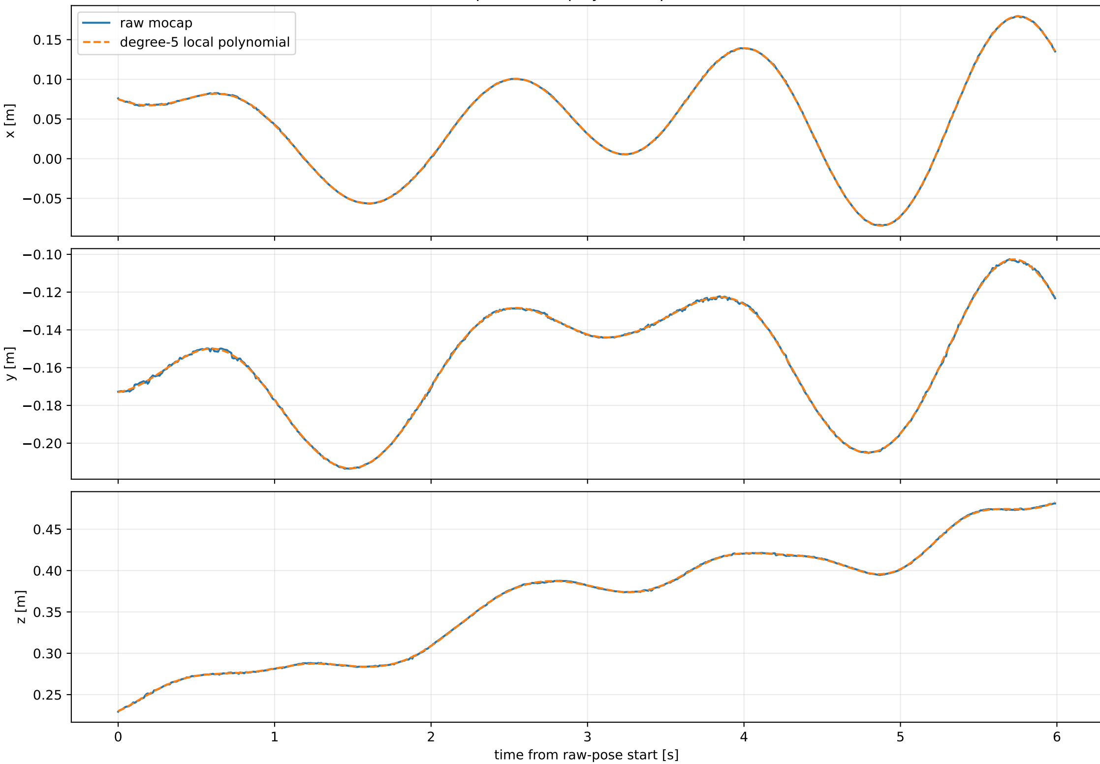
Raw mocap and local-polynomial position; W=1s
