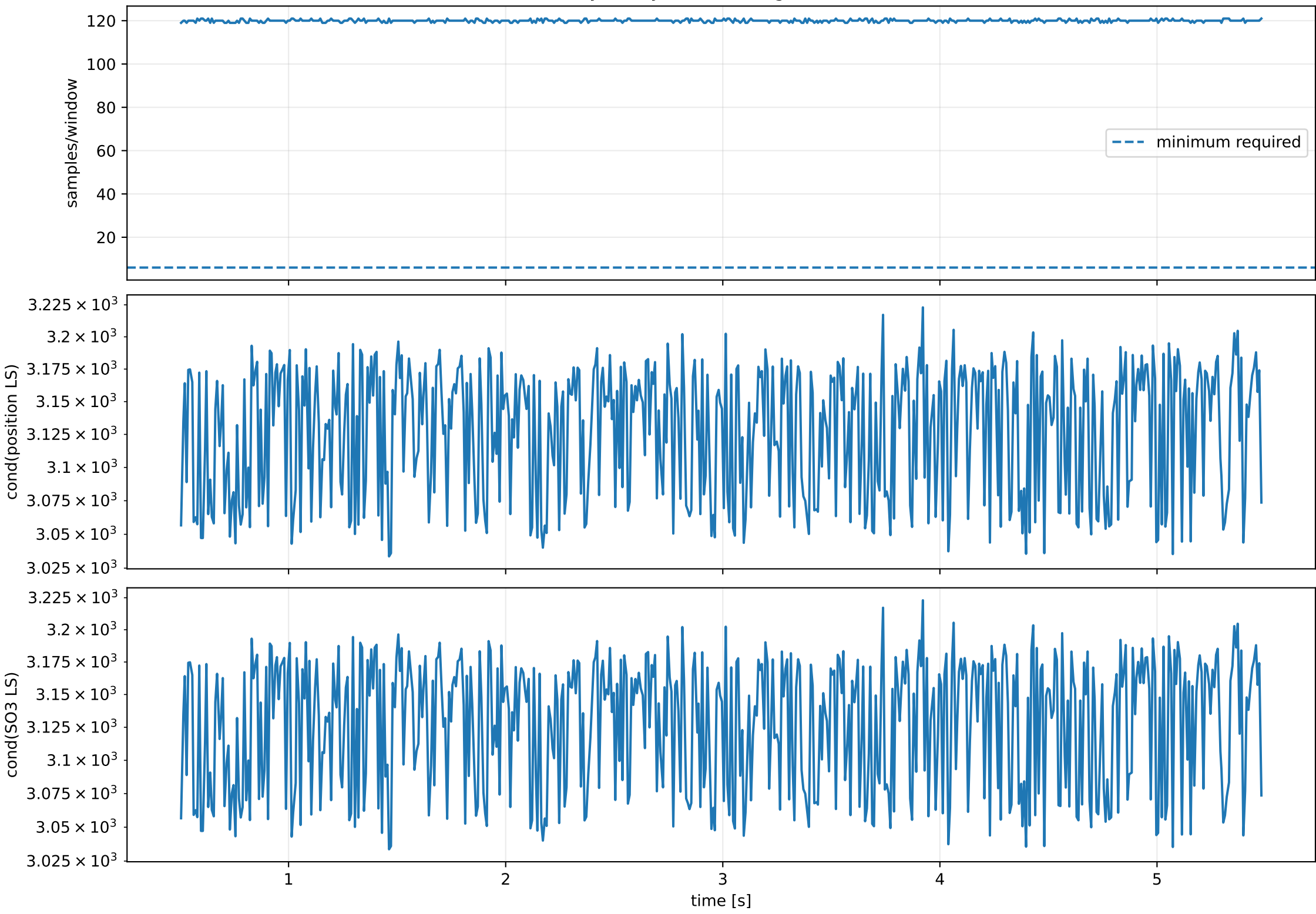
Savitzky-Golay window diagnostics; W=1s
