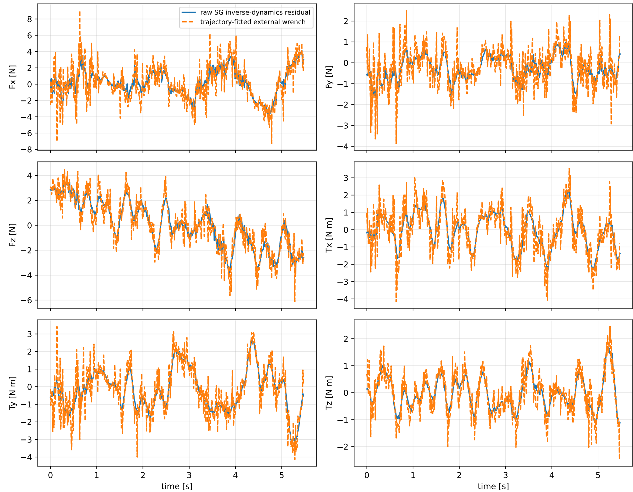
actuator_direct_command: residual wrench
