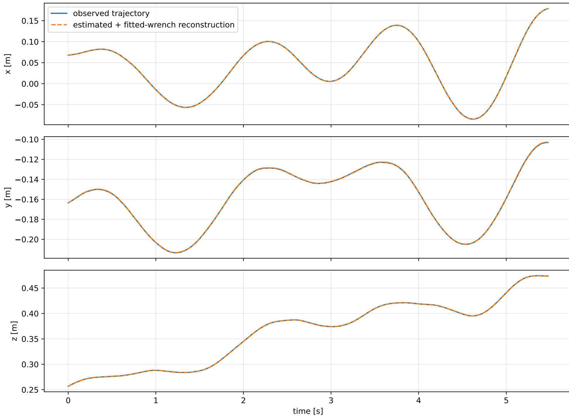
actuator_direct_command: trajectory
