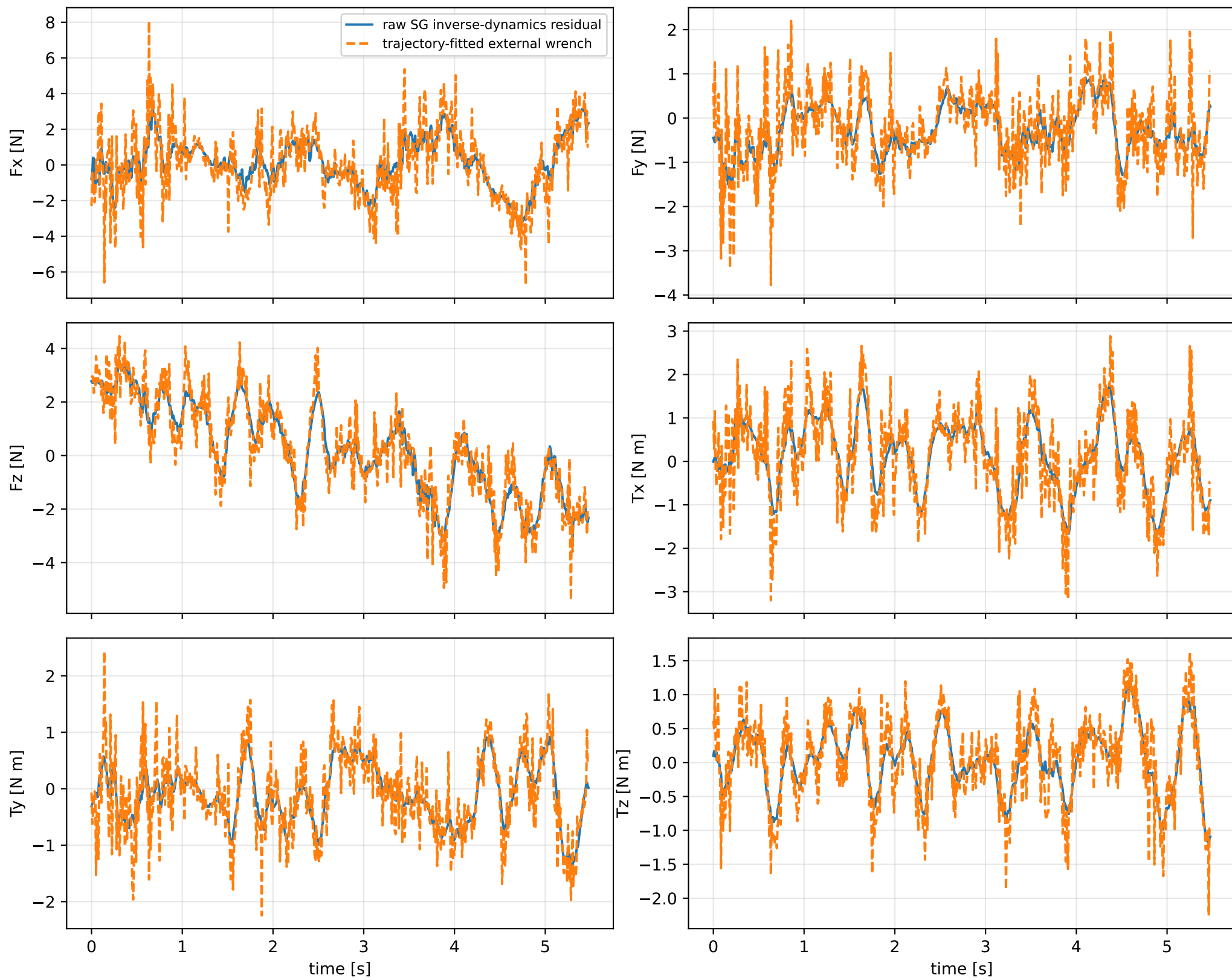
cov_block_s_alpha: residual wrench
