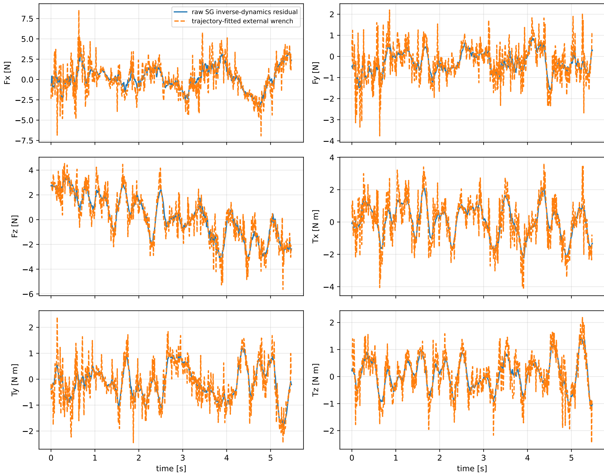
cov_full_no_position_rotation_cross: residual wrench
