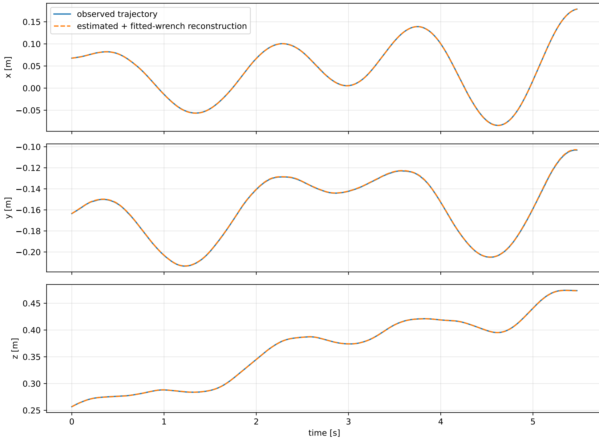
cov_full_no_position_rotation_cross: trajectory
