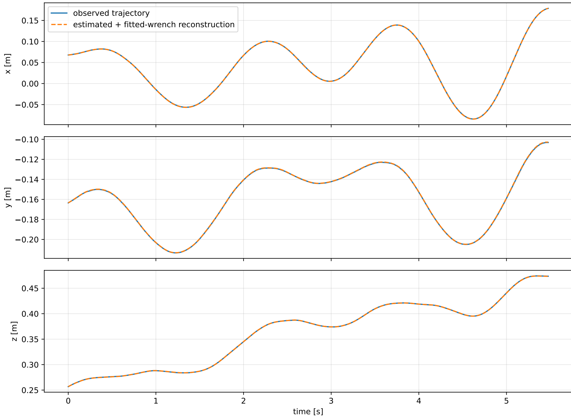
cov_global_full: trajectory
