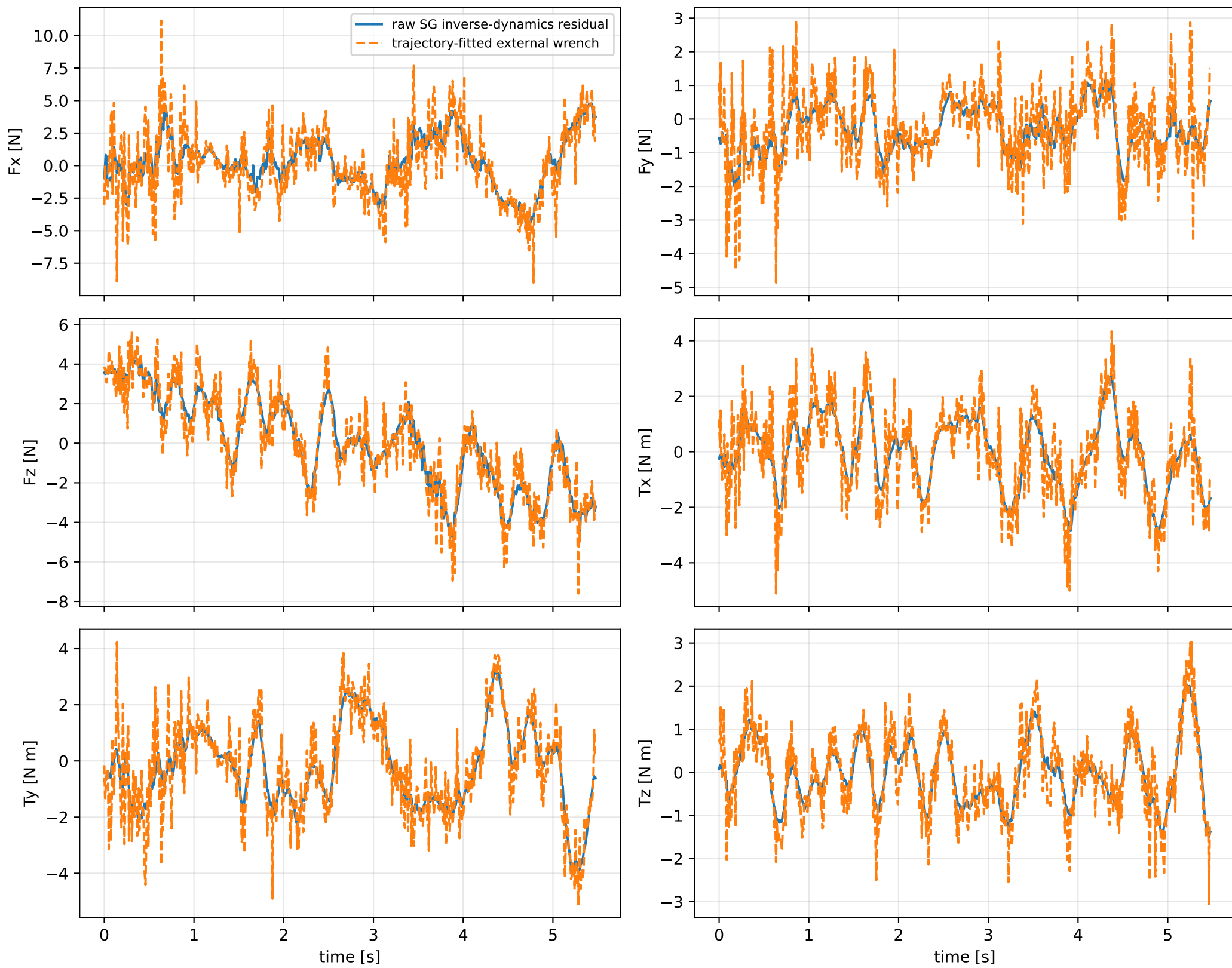
kkt_off_scale_positive: residual wrench
