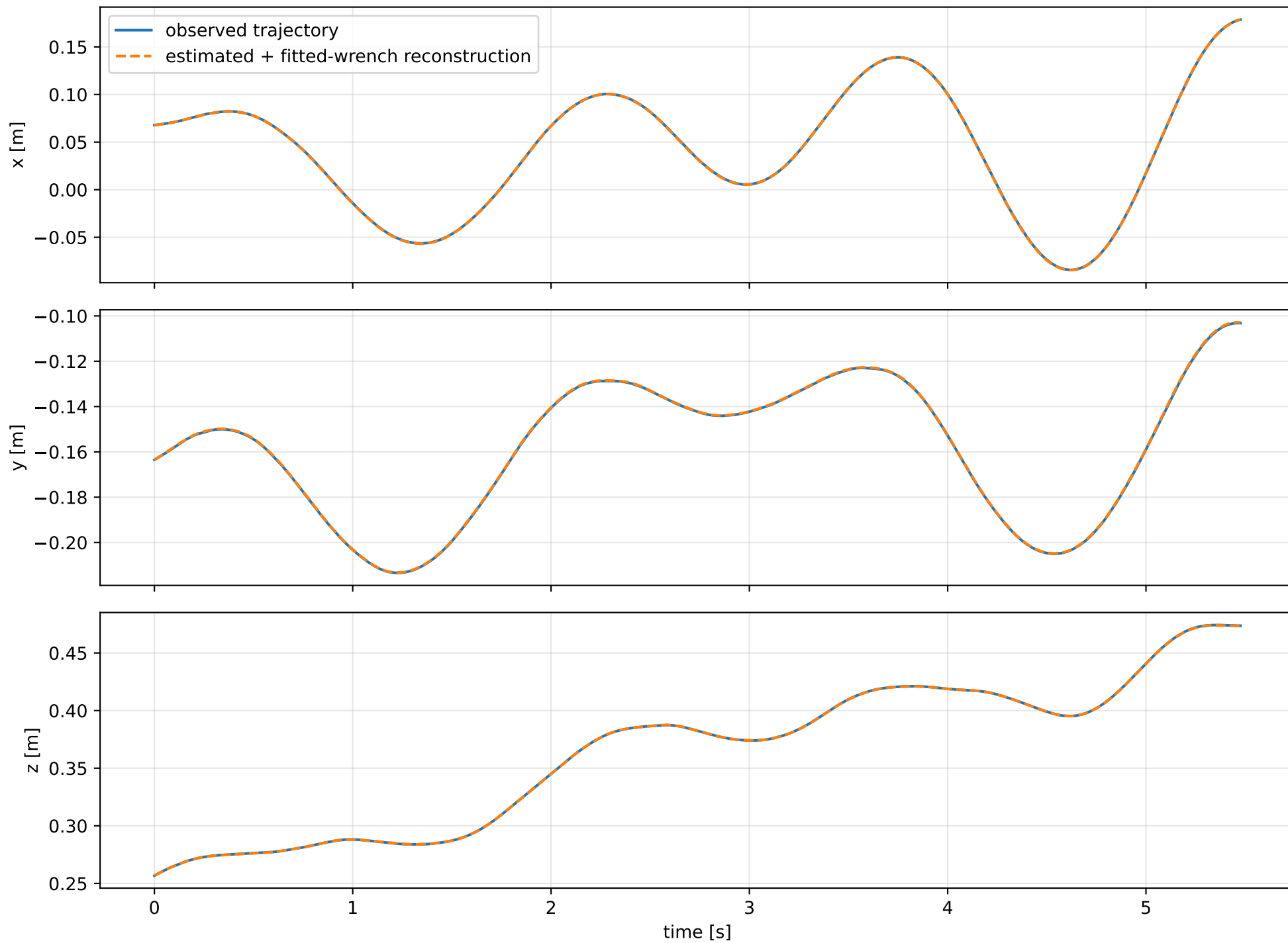
lag_common_estimated: trajectory
