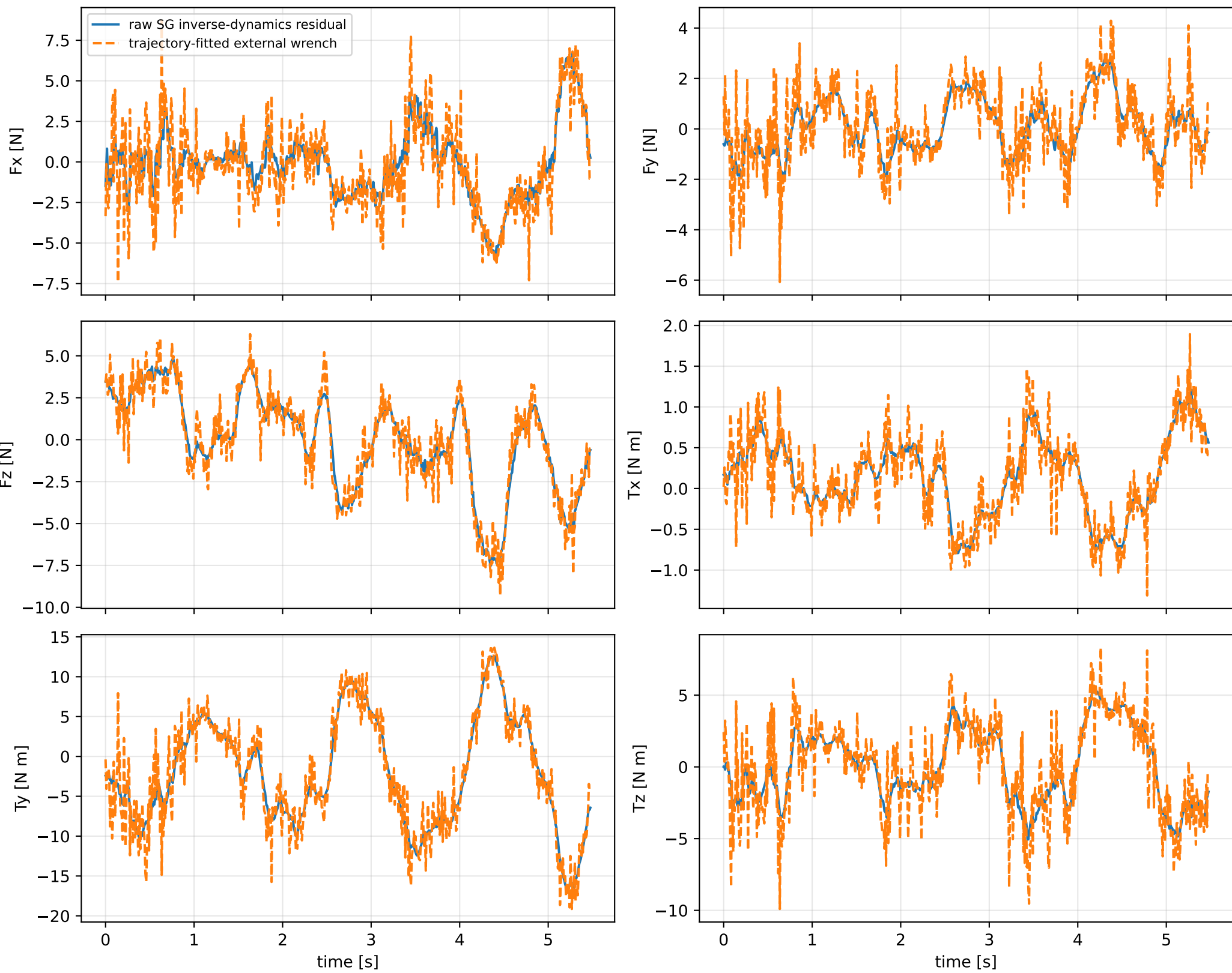
lag_common_estimated: residual wrench
