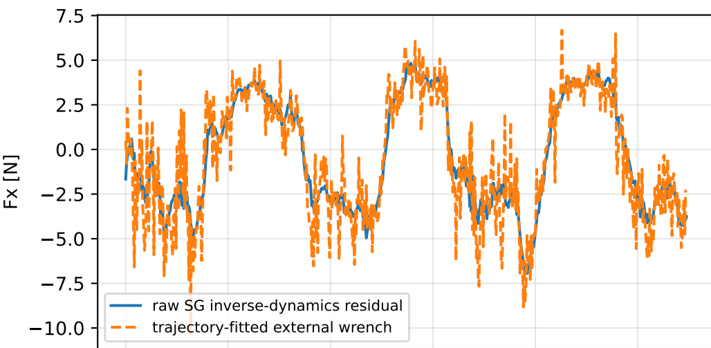
lag_zero: residual wrench
