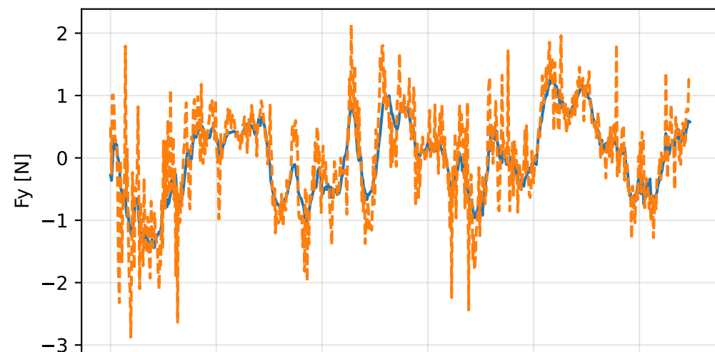
lag_zero: residual wrench
