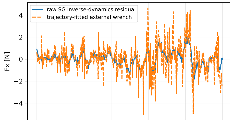
actuator_stateful: residual wrench
