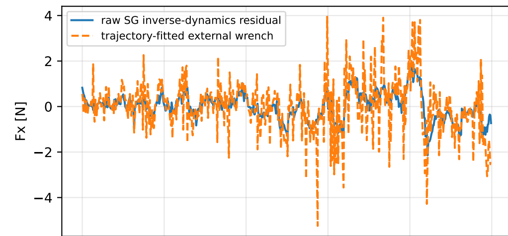
cov_full_no_R_uncertainty_in_s: residual wrench
