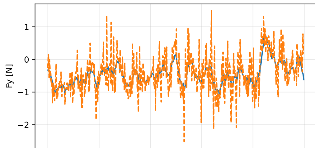
cov_full_no_R_uncertainty_in_s: residual wrench
