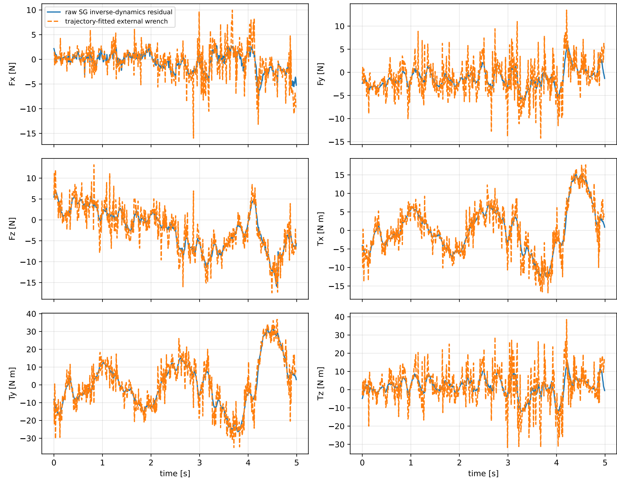
cov_full_no_position_rotation_cross: residual wrench
