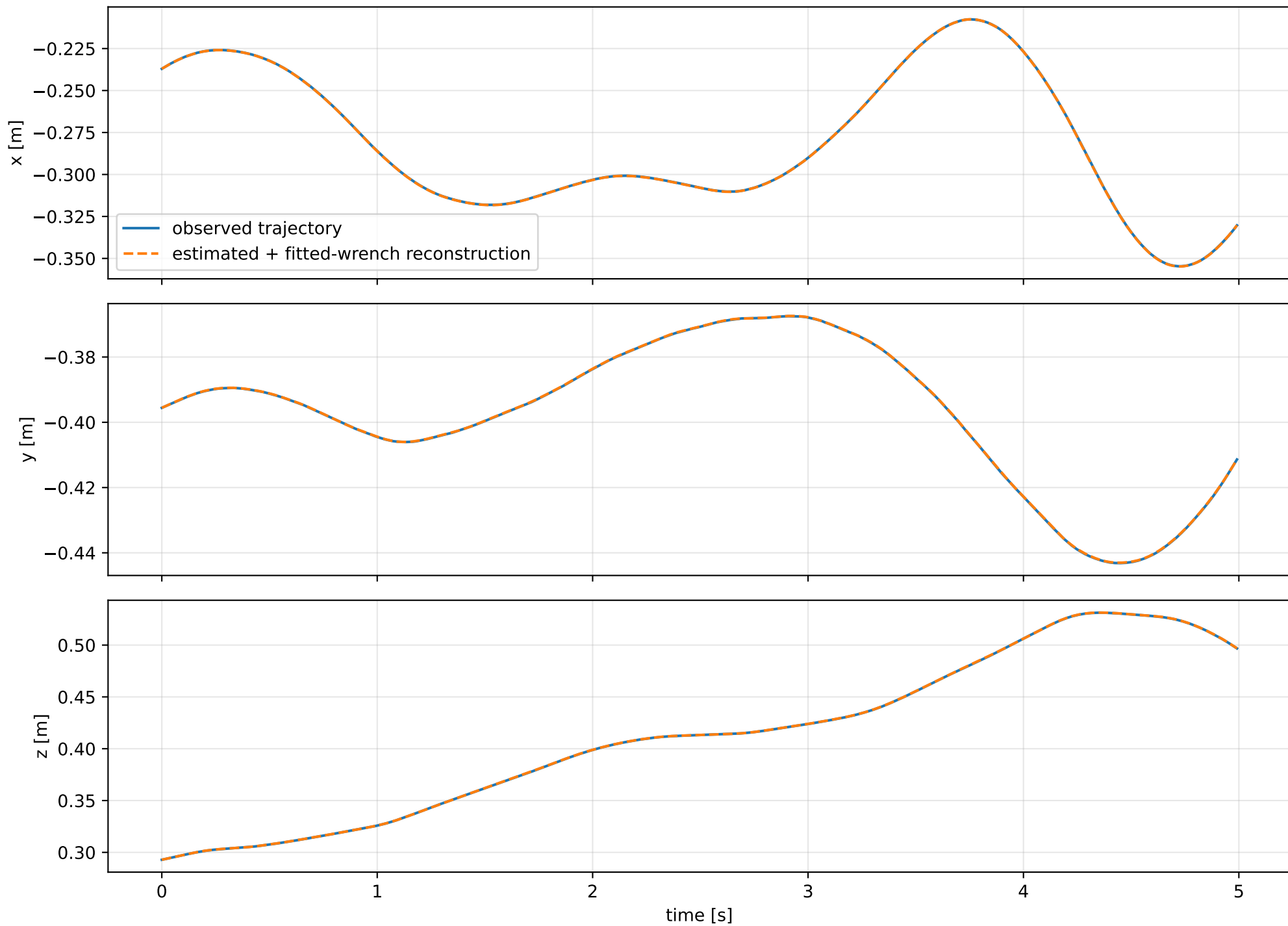
cov_full_no_position_rotation_cross: trajectory
