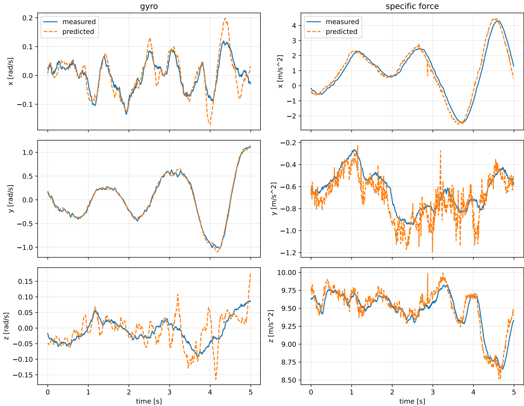
cov_full_no_position_rotation_cross: measured sensor comparison
