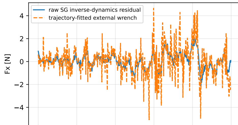
external_wrench_trajectory_fitted: residual wrench
