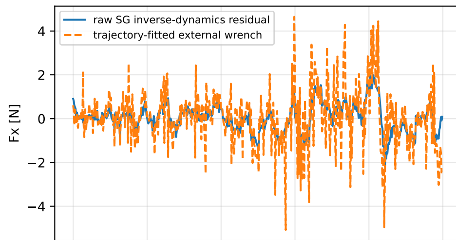
jacobian_analytic: residual wrench
