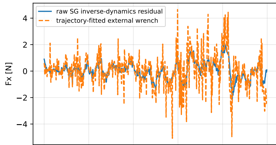
kkt_on_scale_negative: residual wrench
