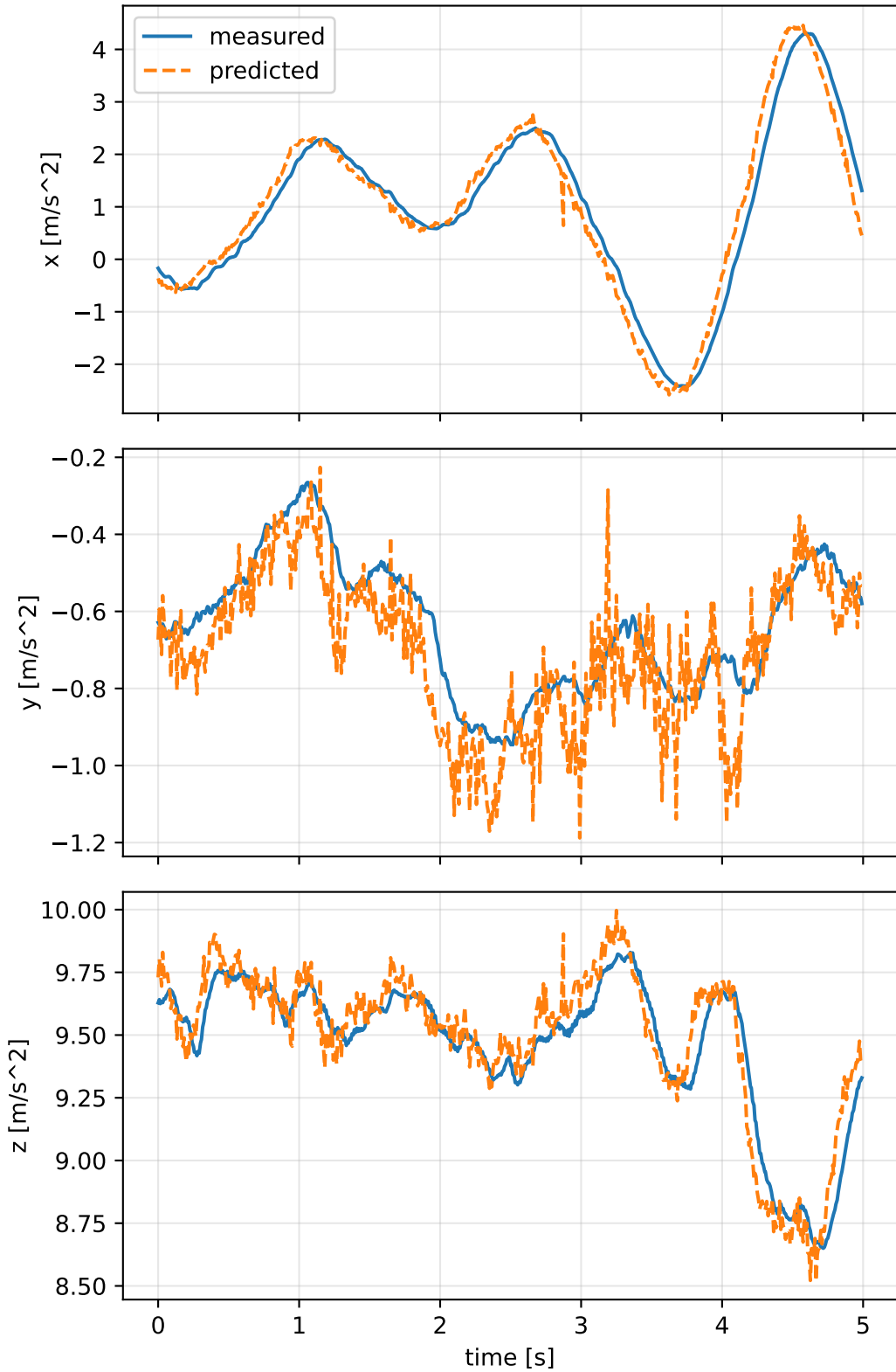
specific force
