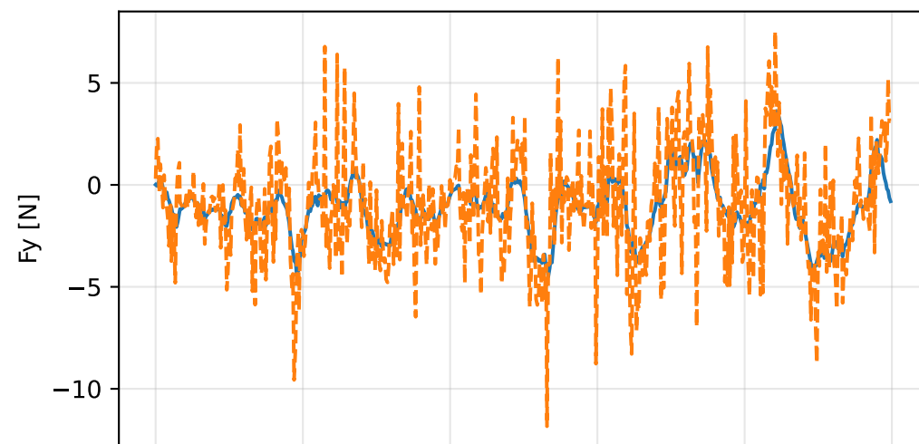
lag_fixed: residual wrench
