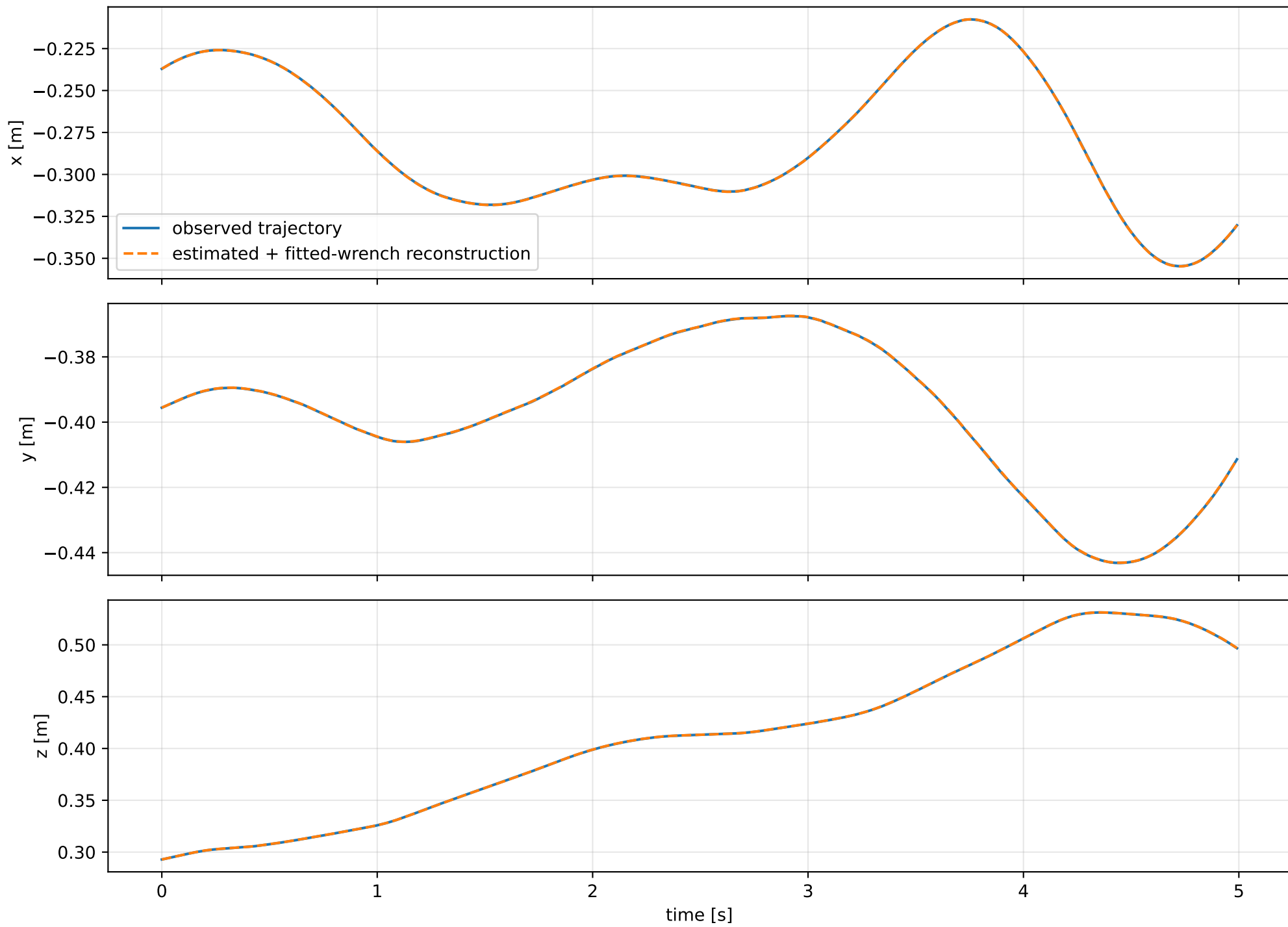
lag_split_strict_only: trajectory
