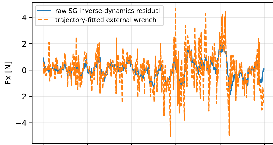
solver_custom_kkt_lm: residual wrench
