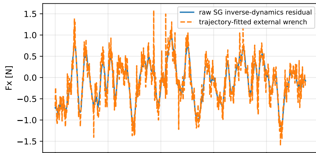
actuator_stateful: residual wrench
