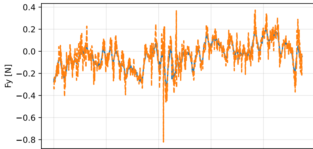
cov_full_no_position_rotation_cross: residual wrench
