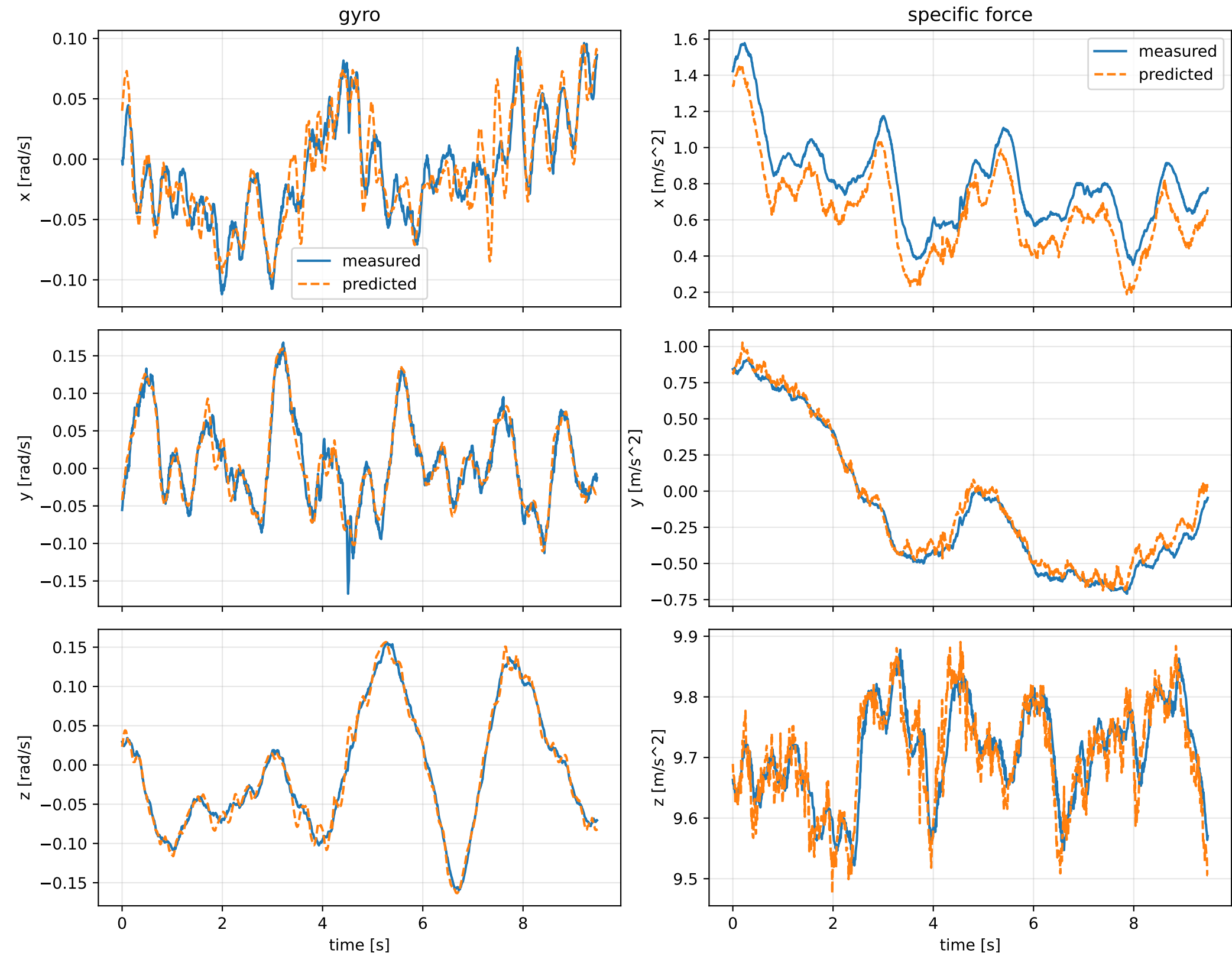
cov_global_full: measured sensor comparison
