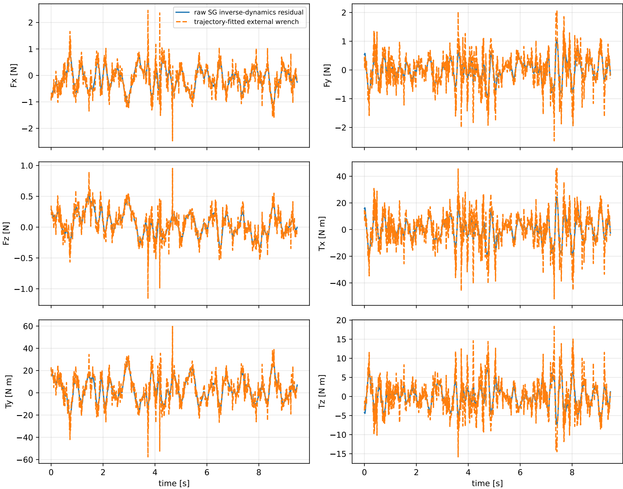
cov_global_full: residual wrench
