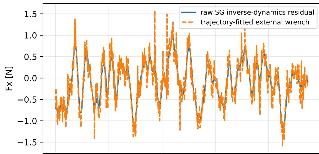
external_wrench_raw_only: residual wrench
