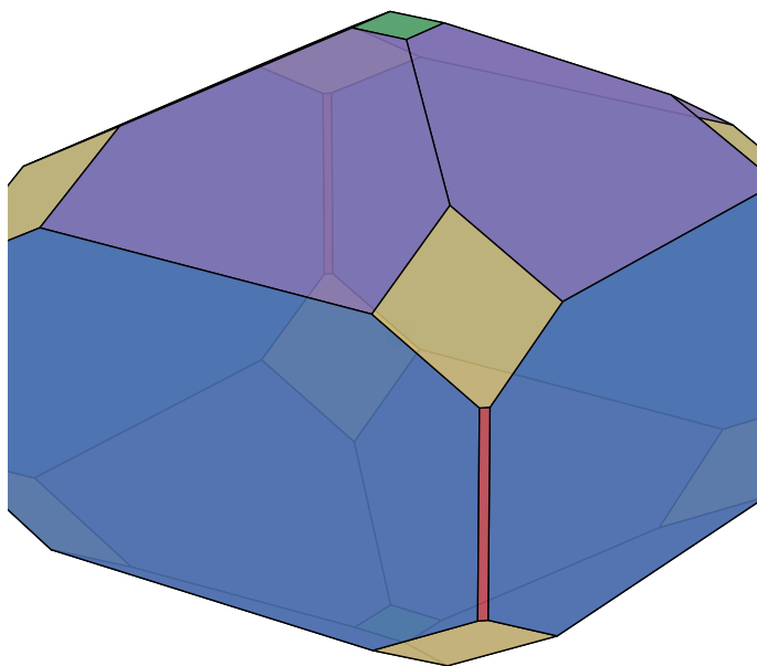
ORB v3 (100):246, (101):231, (110):344, (111):273, (001):250
