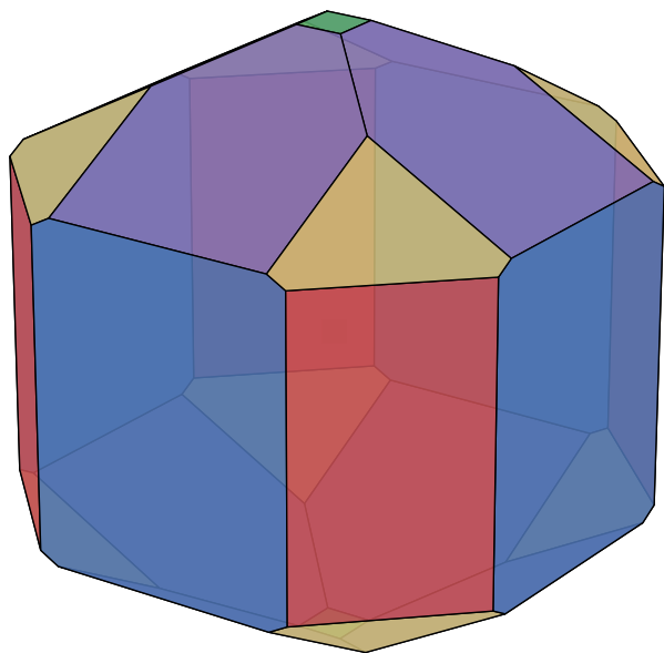
MACE-MPA-0 (100):360, (101):345, (110):461, (111):410, (001):354
