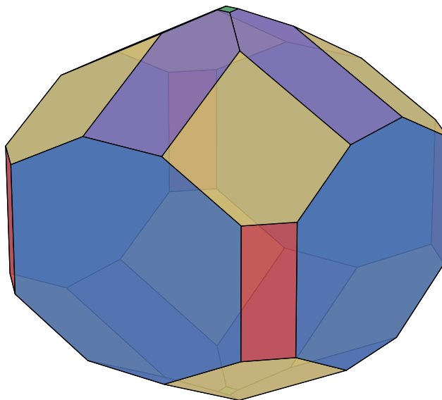
ORB v3 (100):246, (101):231, (110):344, (111):273, (001):250
