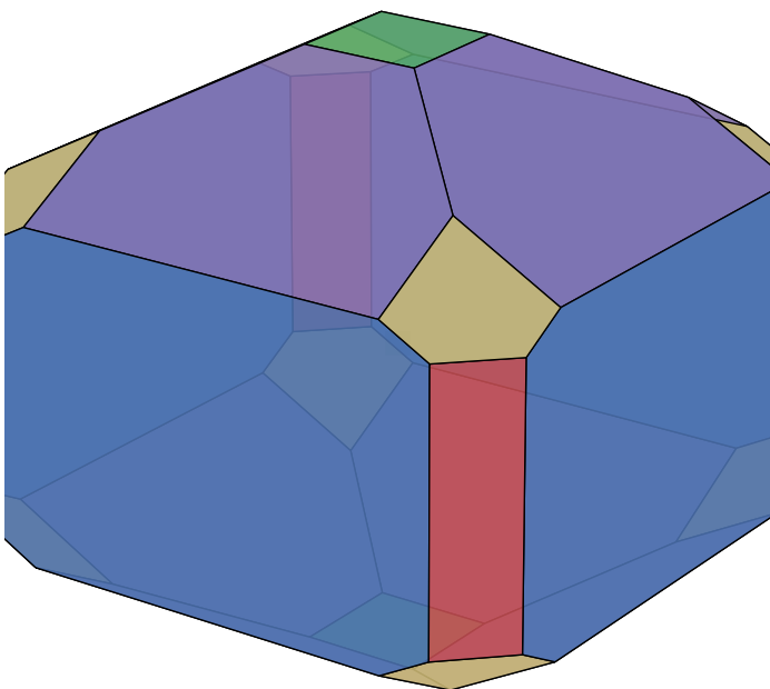
MACE-MPA-0 (100):360, (101):345, (110):461, (111):410, (001):354
