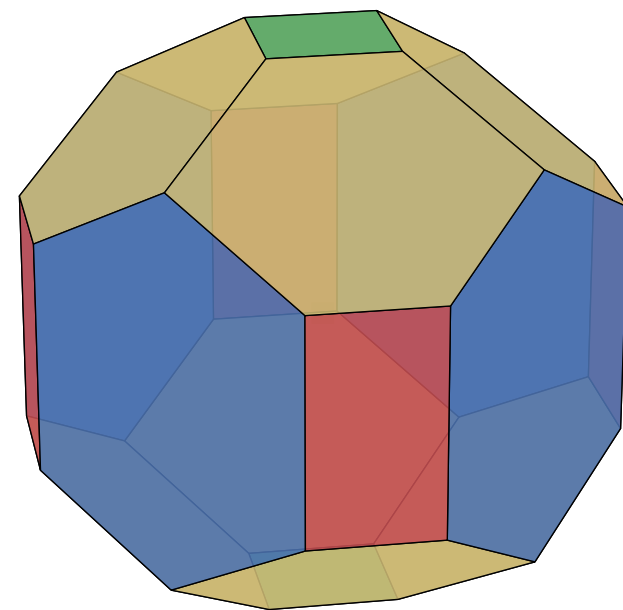
SevenNet-Omni (100):358, (101):365, (110):468, (111):424, (001):375
