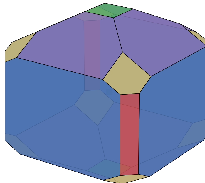
SevenNet-Omni (100):358, (101):365, (110):468, (111):424, (001):375
