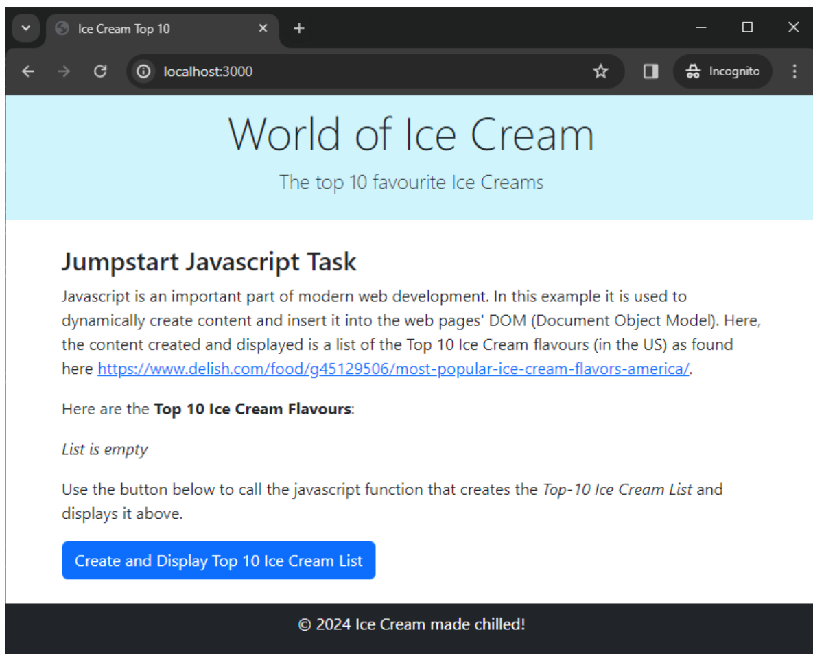
Jumpstart Javascript - Ice Cream List is empty
