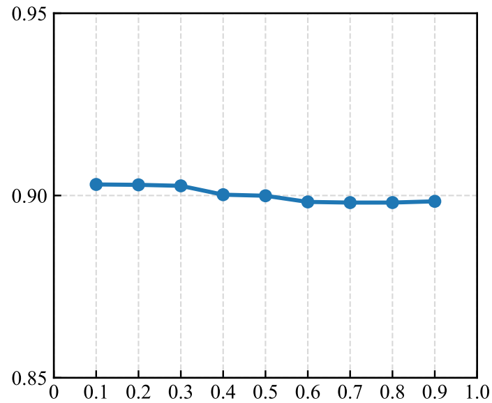
BPIC17
