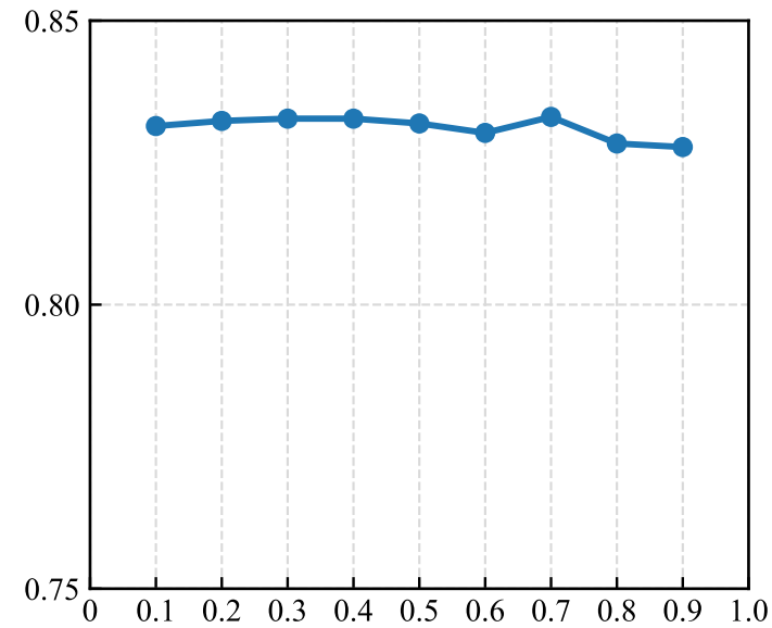
BPIC20PC
