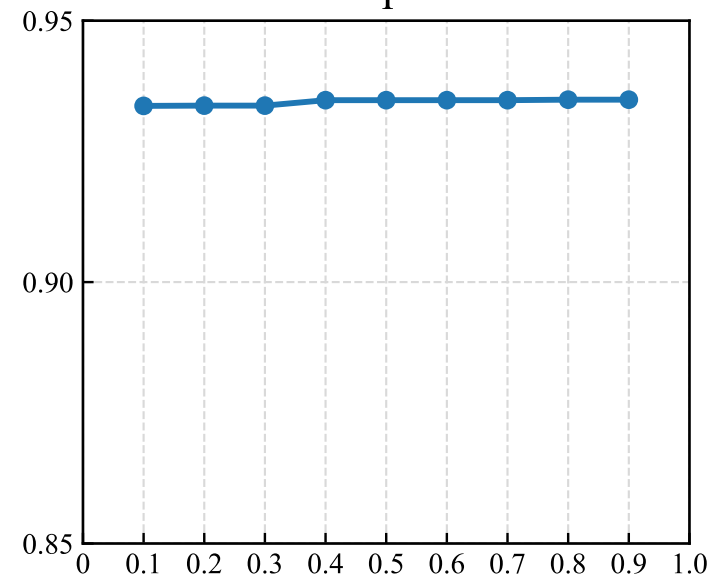
Hospital
