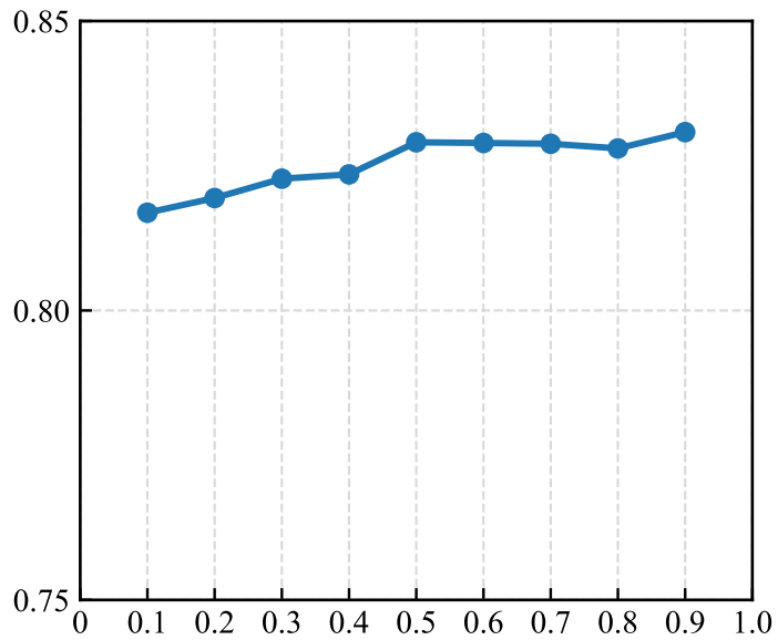
BPIC12
